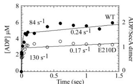
FIG. 4. Substitution of Glu-210 with Asp or Asn impairs rapid binding and hydrolysis of two ATP molecules by SecA dimer. Pre-steady-state acid quench assays were performed with 2.6–3 \mu\text{M} SecA dimer and 500 \mu\text{M} ATP + [ \alpha - ^{32}\text{P} ]ATP (final concentrations) at 37^\circ\text{C} . A, wild type (WT) SecA catalyzes rapid ATP hydrolysis ( \bullet ), with a burst rate constant of 27 \pm 2.5 \text{ s}^{-1} and amplitude 5.2 \pm 0.1 \mu\text{M} (1.8 ATP per dimer), followed by a slow steady-state phase at k_{\text{cat}} = 0.3 \text{ s}^{-1} . In contrast, the SecA-E210N mutant displays no ATP hydrolysis activity in the first catalytic turnover ( \square ). SecA-E210D appears to have residual ATPase activity manifest at a slow linear rate constant of 0.3 \text{ s}^{-1} ( \circ ). B, pulse-chase analysis reveals rapid binding of 2 ATP molecules to the SecA dimer at an apparent binding rate constant of 0.2 \times 10^6 \text{ M}^{-1} \text{ s}^{-1} ( \bullet ; 80–90 \text{s}^{-1} \div 500 \mu\text{M} ). SecA-E210D also binds ATP rapidly ( 0.25 \times 10^6 \text{ M}^{-1} \text{ s}^{-1} ), but the reduced burst amplitude suggests a defect in ATP binding as well as ATP hydrolysis activity.
