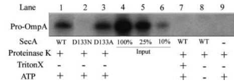
FIG. 6. Aspartate 133 does not appear essential for SecA ATPase and protein translocation activity. A, in endogenous, membrane, and translocation ATPase assays at 37 °C, the SecA-D133N mutant shows poor activity relative to wild type (WT) SecA, but SecA-D133A appears to retain full activity. B, P_i release kinetics in the first turnover reveal that SecA-D133N (black) indeed cannot catalyze ATP hydrolysis, whereas SecA-D133A (gray) retains near wild type ATP binding and hydrolysis activity at 37 °C (burst rate constant = 20 s -1 ; amplitude = 1.6 \mu M; k_{cat} = 0.1 s -1 ). C, correspondingly, no pro-OmpA protein translocation activity can be detected with SecA-D133N in the reaction (lane 2), unlike that observed with SecA-D133A (lane 3) and wild type SecA (lane 1).
