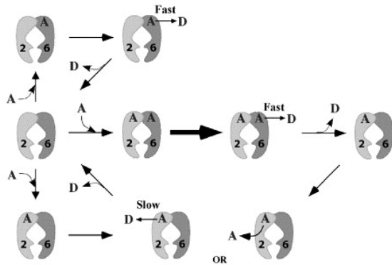
(B) ATP binding to Msh6 is necessary but not sufficient to alter Msh2-Msh6 interaction with DNA
