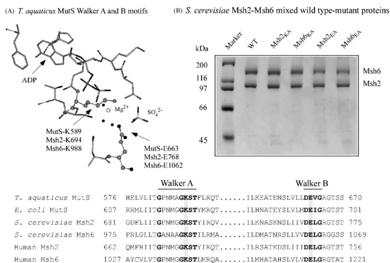
Fig. 1. Msh2, Msh6 Walker A and B motif mutants: (A) ADP, Mg^{2+} , and SO_4^{2-} bound in the conserved ATP binding and hydrolysis site of Thermus aquaticus MutS. (B) Purified mixed wild type–mutant Msh2–Msh6 heterodimers, containing mutations in Msh2 or Msh6 Walker A (Msh2: K694A, Msh6: K988A) and Walker B (Msh2: E768A, Msh6: E1062A) sites.
