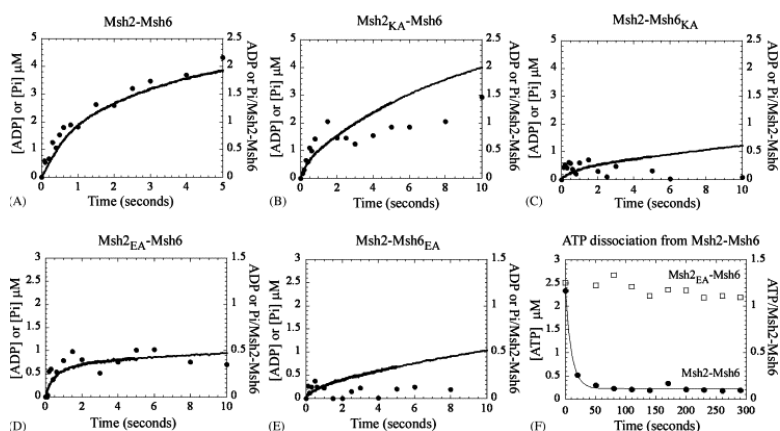
ATPase activity of Msh2-Msh6 in the absence of DNA
