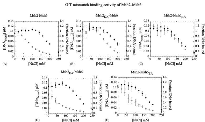
Fig. 5. Msh2–Msh6 binding to mismatched DNA is altered when both subunits bind ATP (ATP \gamma S): interaction of a G:T mismatch with (A) Msh2–Msh6, (D) Msh2 E768A –Msh6 WT , (E) Msh2 WT –Msh6 E1062A dimers (in which both subunits are capable of binding ATP) becomes highly sensitive to NaCl concentration in the presence of ATP \gamma S (o) vs. in the absence of ATP \gamma S (●). In contrast, there is no significant change in the NaCl sensitivity of G:T binding to (B) Msh2 K694A –Msh6 WT and (C) Msh2 WT –Msh6 K988A dimers (in which one subunit is mutated for ATP binding activity), in the presence of ATP \gamma S. (A) A control experiment shows background level interaction between Msh2–Msh6 and matched DNA at all NaCl concentrations (x).
