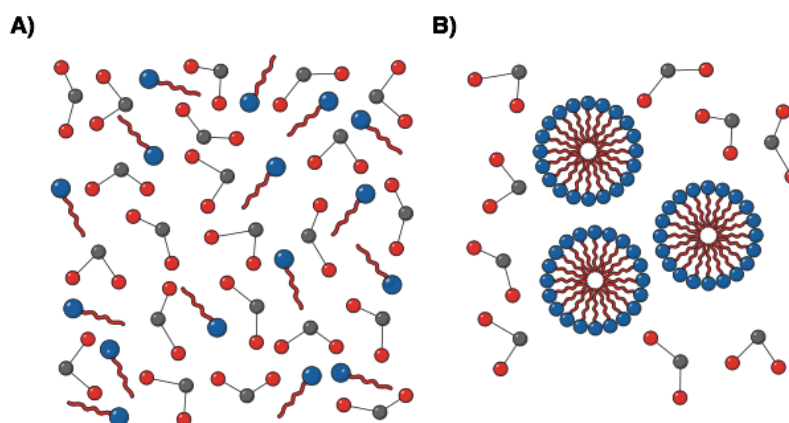
Figure 2.11. Hydrophobic effect and micelle formation. In an aqueous solution, water molecules surround the hydrophobic entities of detergent monomers ( A ). As more of these monomers are added, they self-associate into micelles and the water molecules are dispersed ( B ). 30 Adapted and modified from reference 30.
