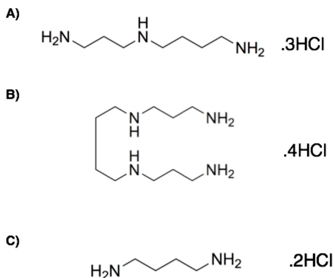
Figure 2.19. Chemical structures of polyamines. Spermidine trihydrochloride ( A ), spermine tetrahydrochloride ( B ), and putrescine dihydrochloride ( C ) can be added to the solubilization buffer that contains a detergent. The structures were constructed using the ChemDraw molecular editor.
