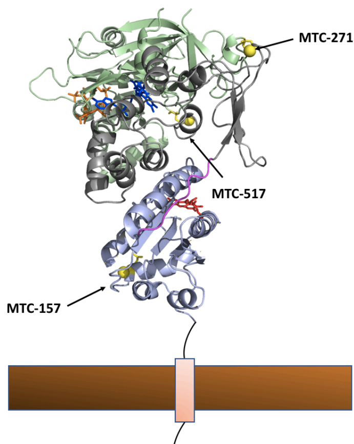
Figure 3.6. Localization of methyl probes on a model for membrane-bound CYPOR. MTC-157 is in the FMN domain, while MTC-271 and MTC-517 are in the FAD/NADP(H) domain of the protein.
