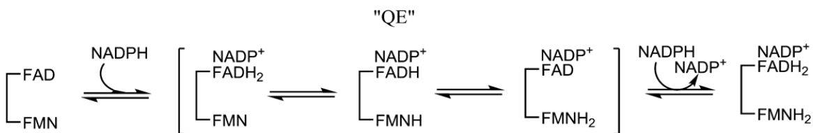
Scheme 1.1. Chemical mechanism of electron transfer in CYPOR. NADPH binds to the protein and delivers a hydride ion to its FAD cofactor, which delivers the electrons one at
