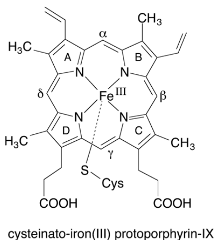
Figure 1.5. Structure of iron (III) protoporphyrin-IX in CYP. 12 \text{Fe}^{\text{III}} in this heme is attached to the sulfur atom of a cysteine residue in CYP. Figure from reference 12.
