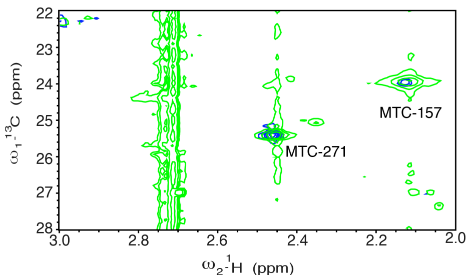
Figure 3.19. Overlay of ^1\text{H} - ^{13}\text{C} HSQC spectra of the Q157C/N271C \Delta 56 CYPOR before (blue) and after (green) the additional ^{13}\text{C} -MMTS.
