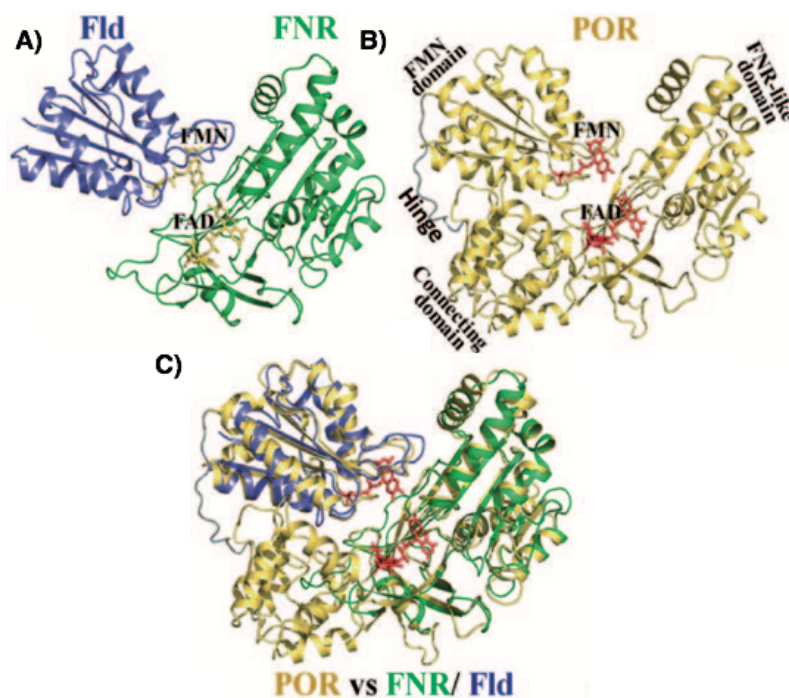
Figure 1.3. Structures of Fld, FNR, and CYPOR. Structures of Fld and FNR ( A ) are similar to the FMN and FNR-like domains of CYPOR ( B ). An overlay of these structures ( C ) confirms this fact. FAD and FMN cofactors are depicted as stick models; those bound to Fld and FNR are colored yellow, while those bound to CYPOR are colored red. Note: in this figure, CYPOR is referred to as “POR”. 1 Adapted from reference 1.
