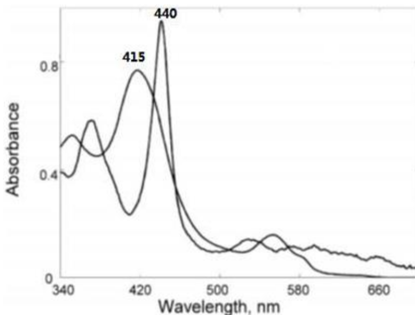
Figure 66 Absorption Spectra for P450cam before (oxy 415 nm) and after (peroxo, hydroperoxo 440 nm) cryoradiolysis 117
