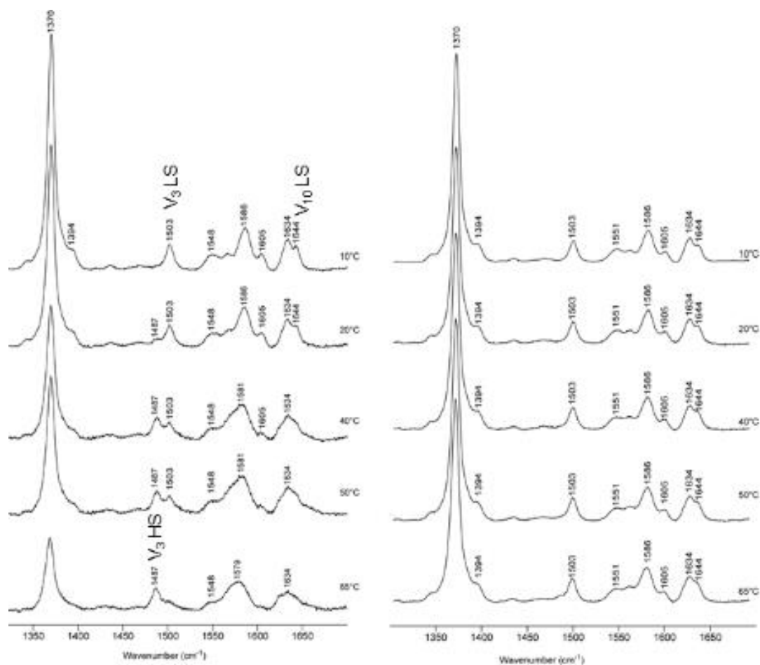
Figure 74 High frequency resonance Raman spectra showing effect of temperature on binding of lauric acid (left) ( \approx 80\% high spin formed at 65^\circ\text{C} ) and effect of temperature on substrate free CYP119 (right) ( \approx 3\text{-}5\% high spin formed at 65^\circ\text{C} )
