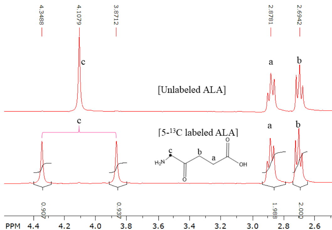
Figure 23 1 H NMR Comparing labeled to unlabeled ALA
