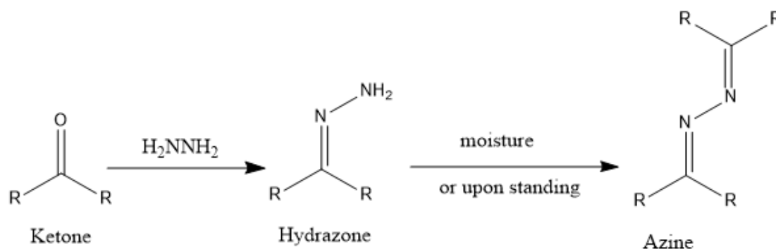
Figure 42 Synthesis of hydrazone scheme showing how the reaction is complicated by formation of azine a stable side product.
