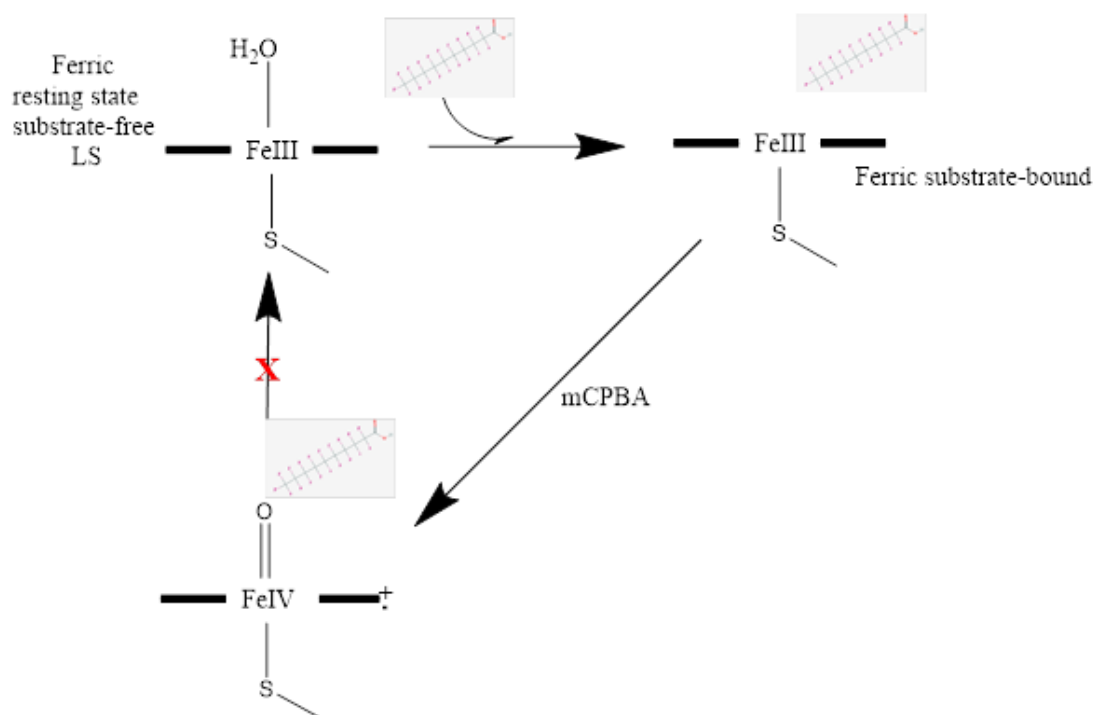
Figure 57 The formation of compound I through the peroxide shunt pathway, oxidizing ferric PFDA bound protein with 3-chloroperoxybenzoic acid (mCPBA)
