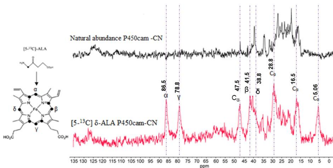
Figure 30 ^{13}\text{C} NMR for natural abundance and [ 5\text{-}^{13}\text{C} ] \delta -ALA P450cam 80 acquired at 25 °C
