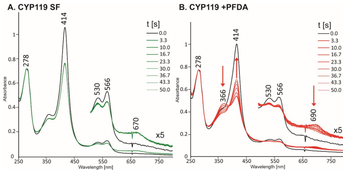
Figure 84 UV-visible spectra for substrate free (left) and PFDA bound CYP119 (right) showing the generation and stabilization of CYP119-I using 5-fold excess mCPBA. CYP119-I lifetime prolonged for up to 45 s. A portion of the protein was also degraded from using excess mCPBA.
