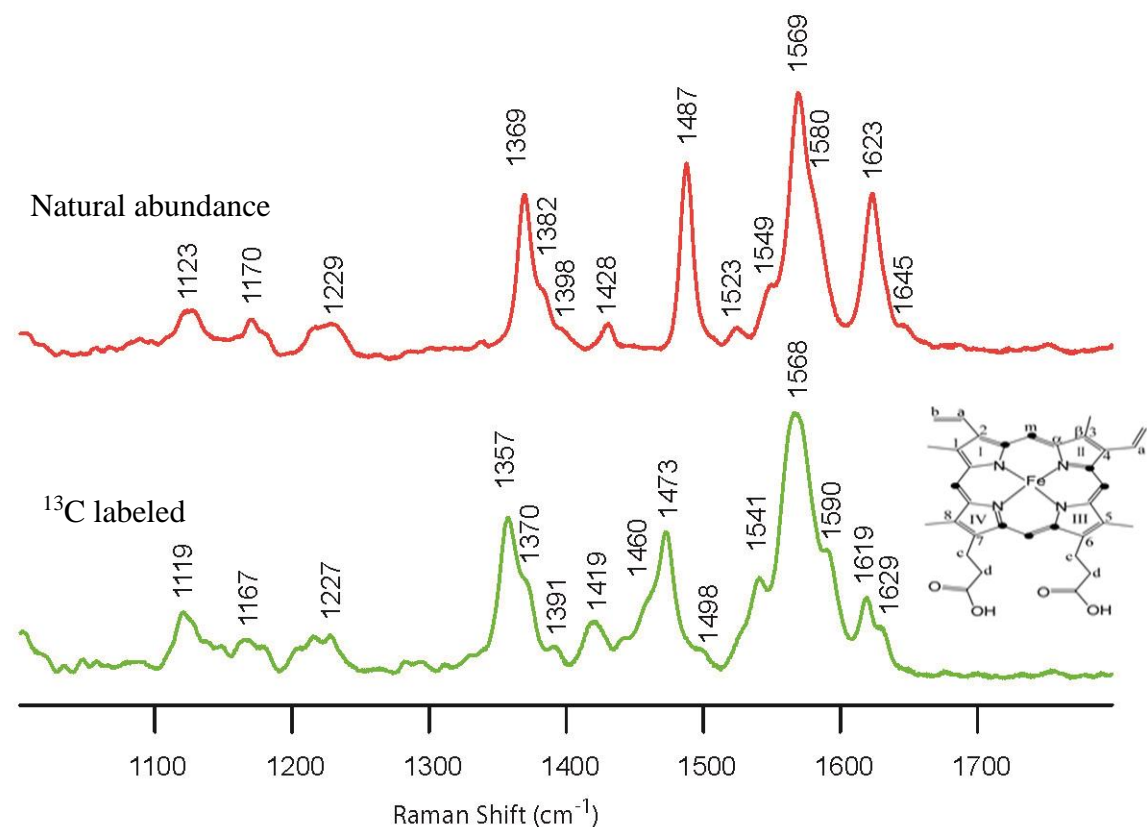
Figure 27 High frequency RR spectrum of CYP101 13 C labeled relative to the natural abundance CYP101
