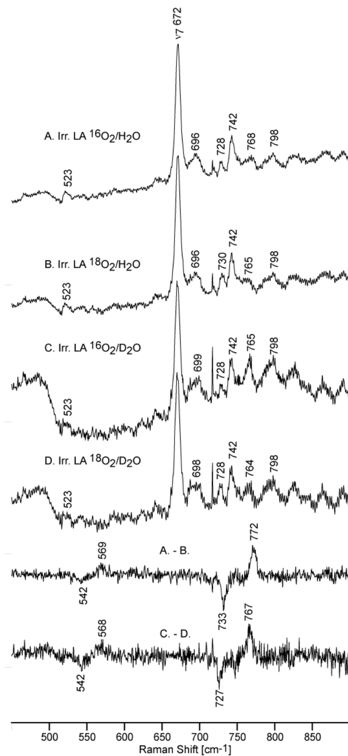
Figure 81 Middle frequency rR spectra of oxy CYP119 with LA after irradiation; A) ^{16}\text{O}_2/\text{H}_2\text{O} , B) ^{18}\text{O}_2/\text{H}_2\text{O} , C) ^{16}\text{O}_2/\text{D}_2\text{O} , D) ^{18}\text{O}_2/\text{D}_2\text{O} , and their difference traces. Total collection time was 6 hours for each spectrum using 442 nm excitation line at 77 K.
