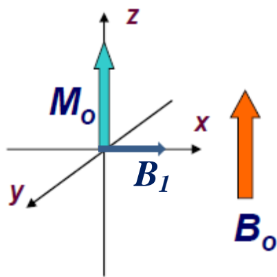
Figure 11 NMR signal obtained after application of a magnetic field
