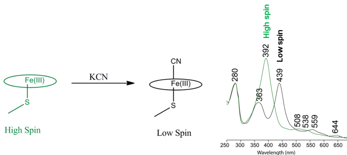
Figure 28 UV-visible absorption spectra for the high spin and low spin complexes of P450cam 80
