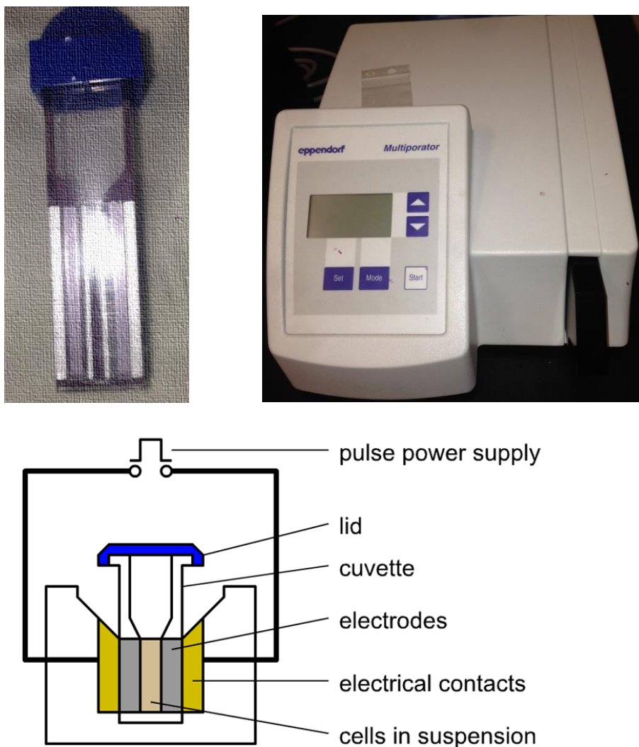
Figure 19 Electroporation cell (left), multiporator (right) for incorporation of second plasmid and details about the electroporation process (bottom)
