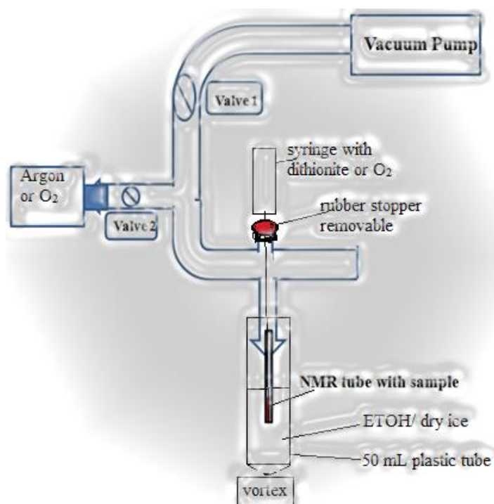
Figure 64 The schematics of vacuum line for preparation of oxy-CYP119 samples.
