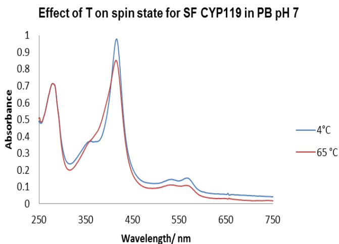
Figure 72 Effect of Temperature on spin state for substrate free CYP119 in 100 mM PB at pH 7
