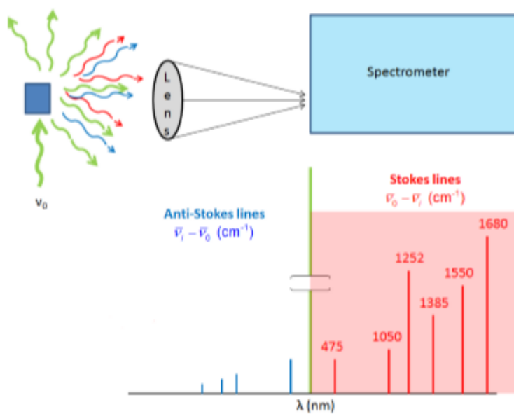
Figure 8 Raman scattering spectroscopy
