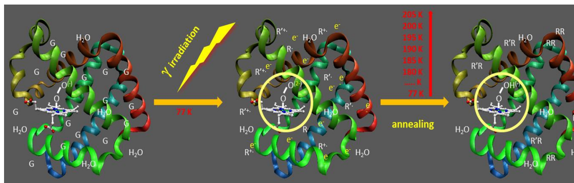
Figure 60 The scheme of cryoradiolytic reduction of ferrous dioxygen adduct (left), to form peroxo (center) and hydroperoxo (right) intermediates upon \gamma irradiation and annealing, respectively
