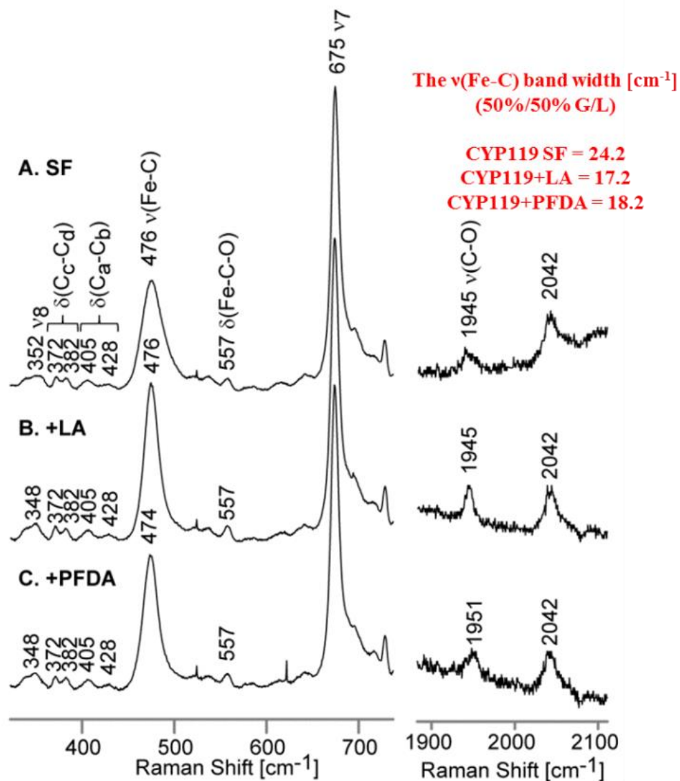
Figure 76 Low frequency (left) and high frequency (right) resonance Raman spectra of ferrous CO adducts of CYP119 and effect of substrates LA and PFDA at 10 °C.
