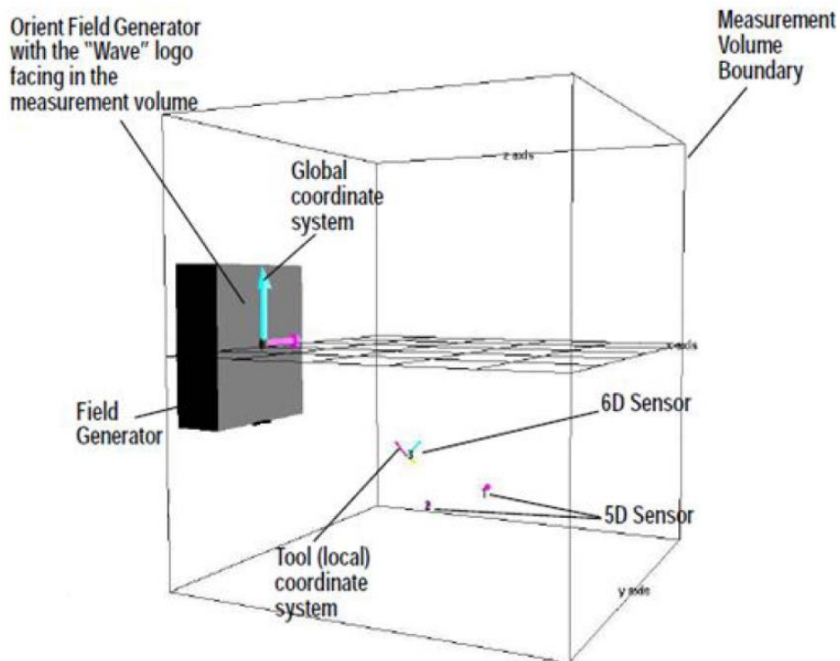
Figure 3: NDI Wave System Field Generator [4]
