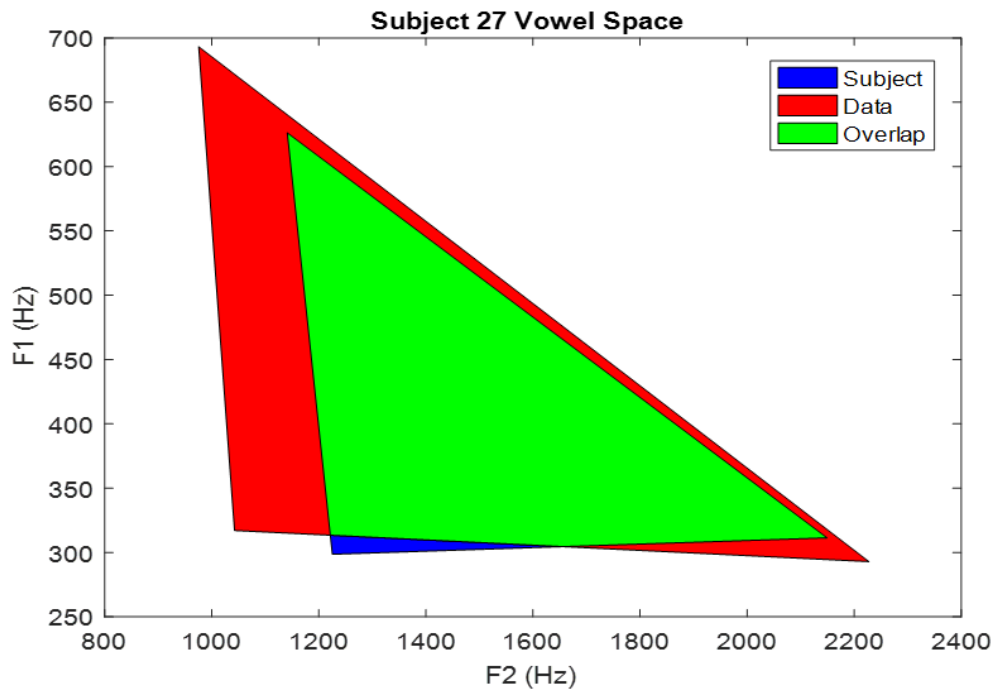
Figure 20: Vowel-Space-Overlap Method
