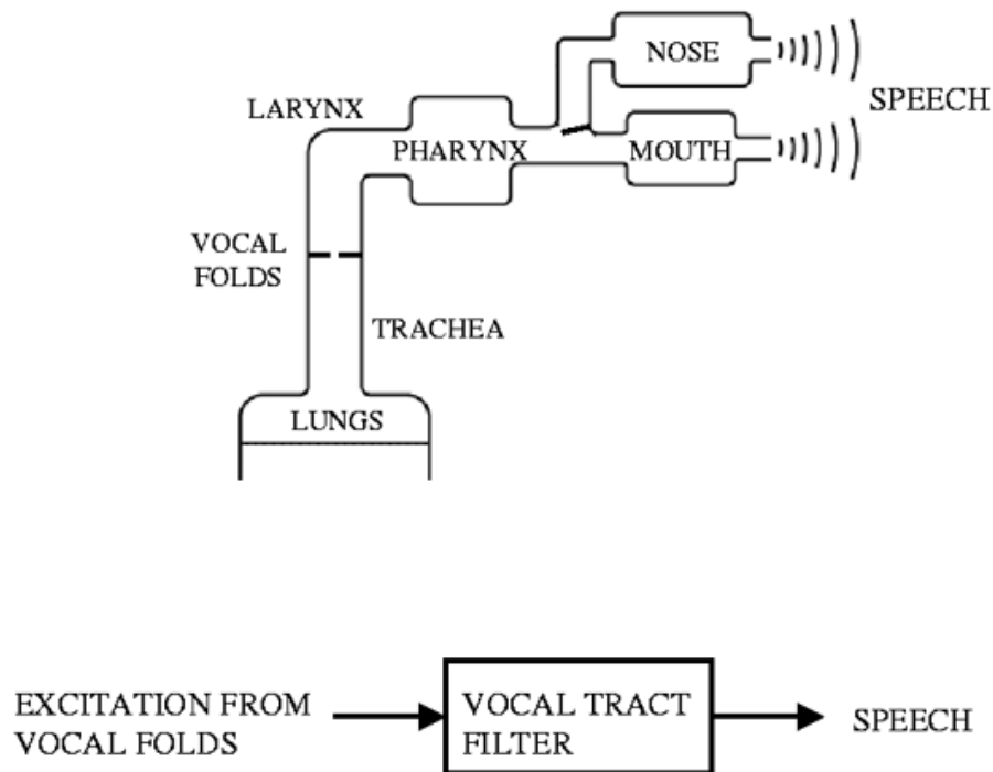
Figure 8: Source-Filter Model [4]
