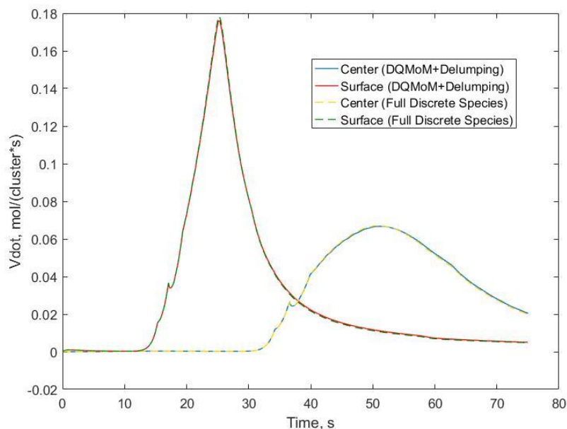
Figure 5-38. Comparison of \dot{V} at the center and surface of 4.5mm radius particle for two models.
