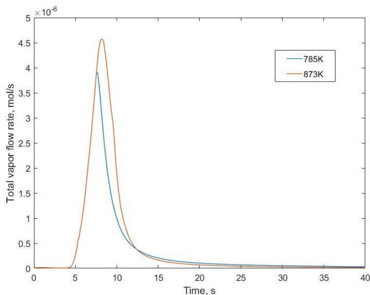
Figure 5-28. Total vapor flow rate of species out of the particle for the whole 0.8mm radius particle versus time at 785K and 873K
