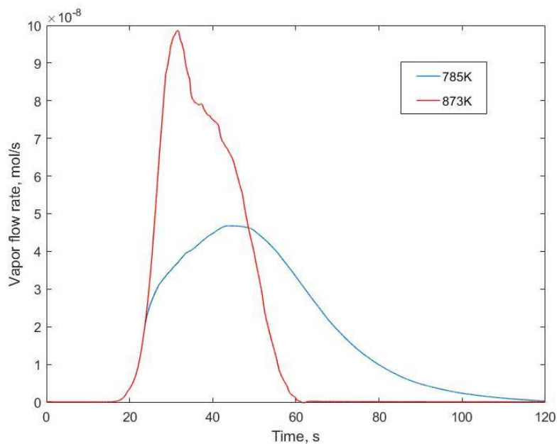
Figure 5-33. Vapor flow rate of species (Molecular Weight 150 kg/kmol) out of the particle for the whole 4.5 radius particle versus different times at 785K and 873K
