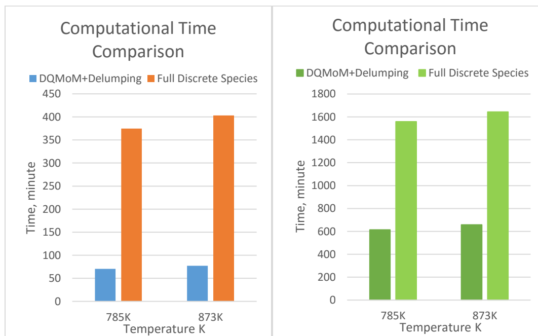
Figure 5-46. Comparison of Computational time for (1) 0.8mm radius particle for different temperatures. (2) 4.5mm radius for different temperatures.
