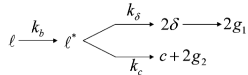
Figure 3-1. Chemical Reaction Scheme in the CPD model
