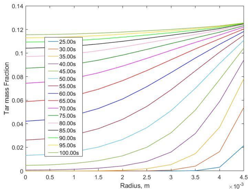
Figure 5-10. The change of mass fraction of tar versus position at particular time for the 4.5mm radius of coal particle with 785K highest temperature
