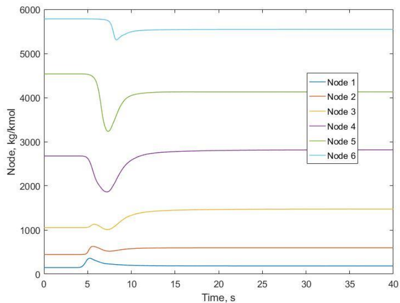
Figure 5-40. Evolution of node at the center of 0.8mm radius particle for DQMoM model.
