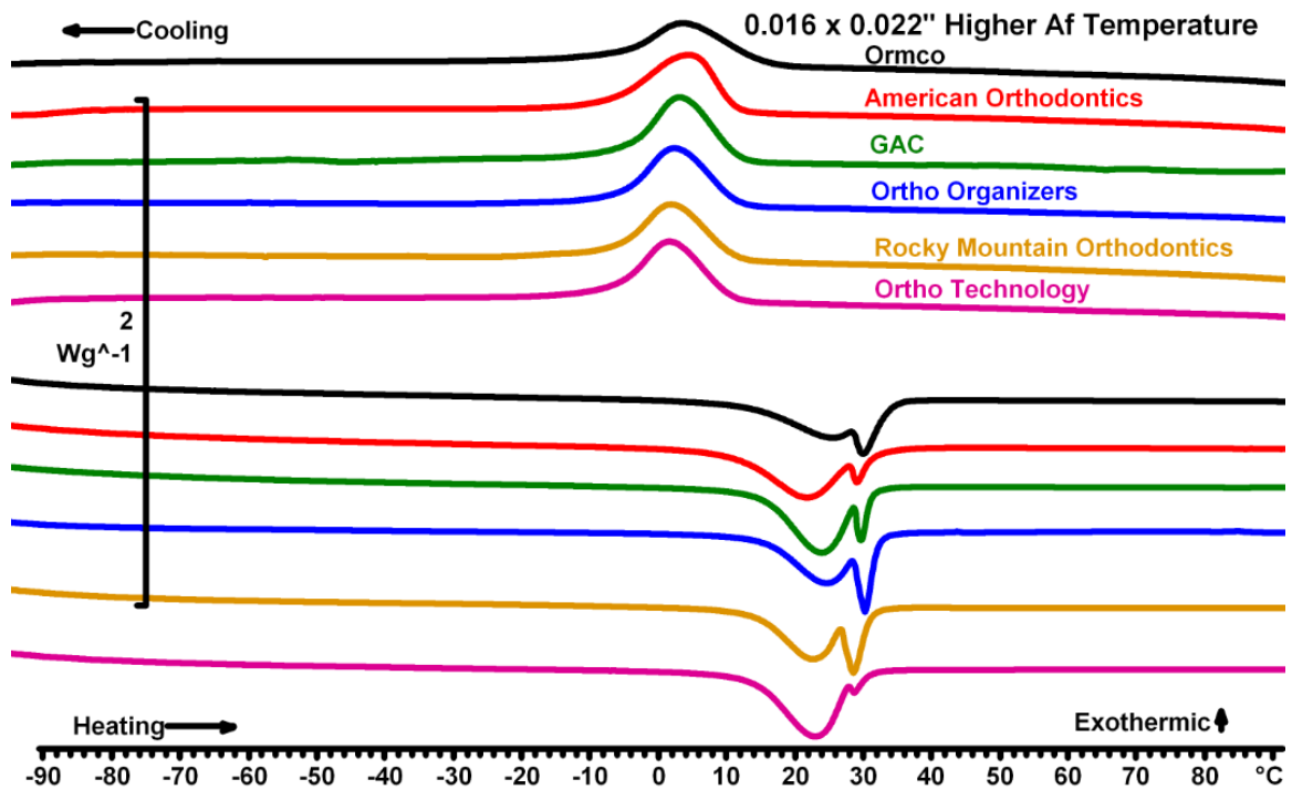
Figure 10: Thermogram for 0.016" x 0.022" wires with Af of 35°C
