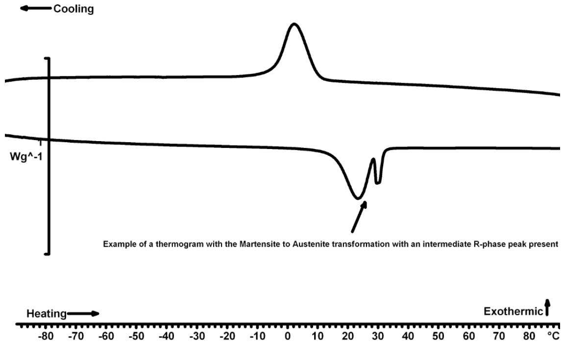
Figure 6: Example of DSC Thermogram with presence of R Phase
