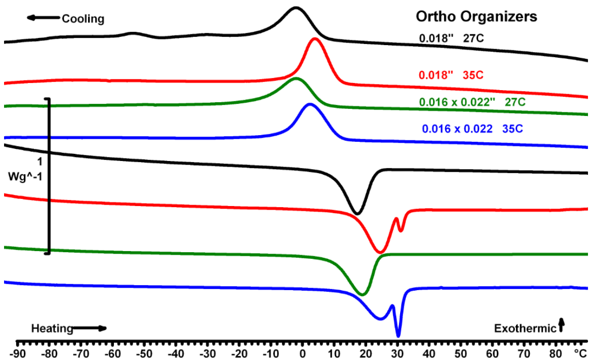
Figure 12: Thermogram for all variants of Ortho Organizers CuNiTi wires
