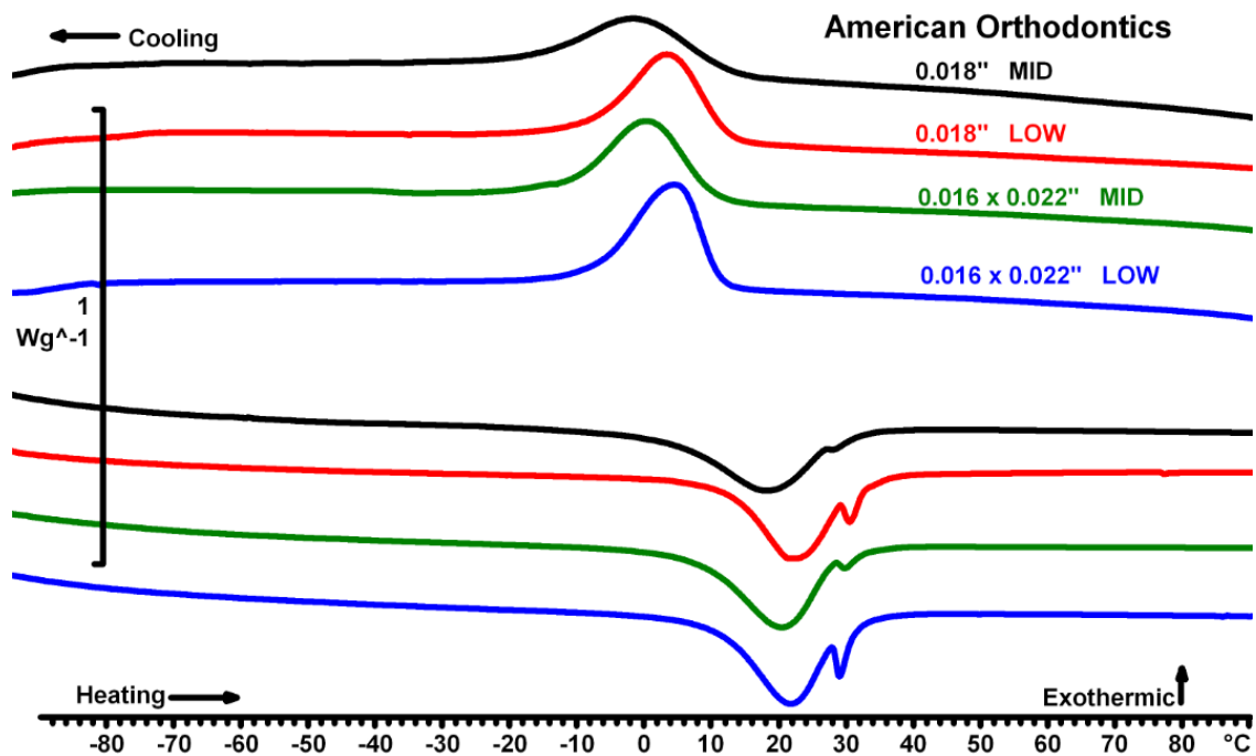
Figure 15: Thermogram for all variants of American Orthodontics CuNiTi wires
