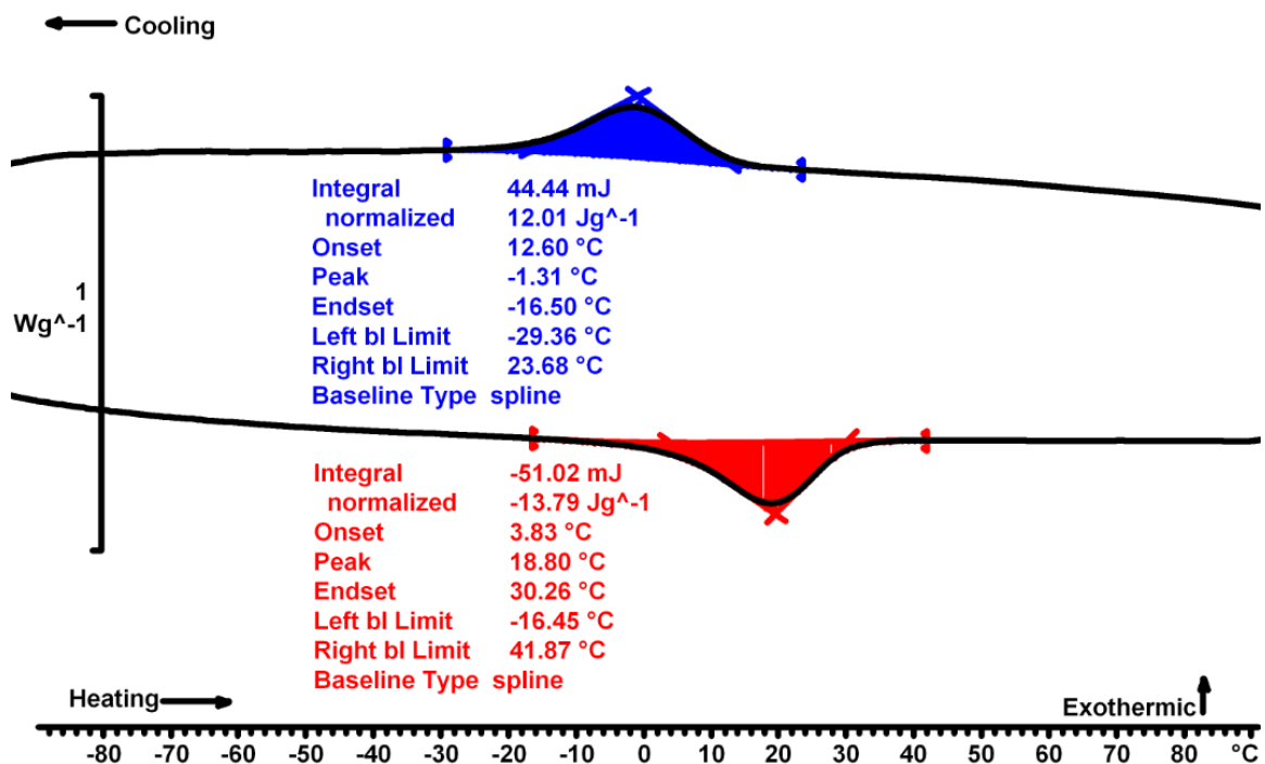
Figure 5: Example of DSC Thermogram Analysis
