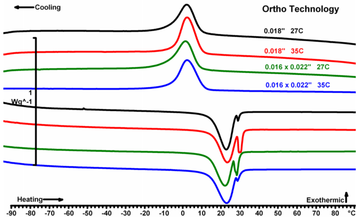
Figure 11: Thermogram for all variants of Ortho Technology CuNiTi wires
