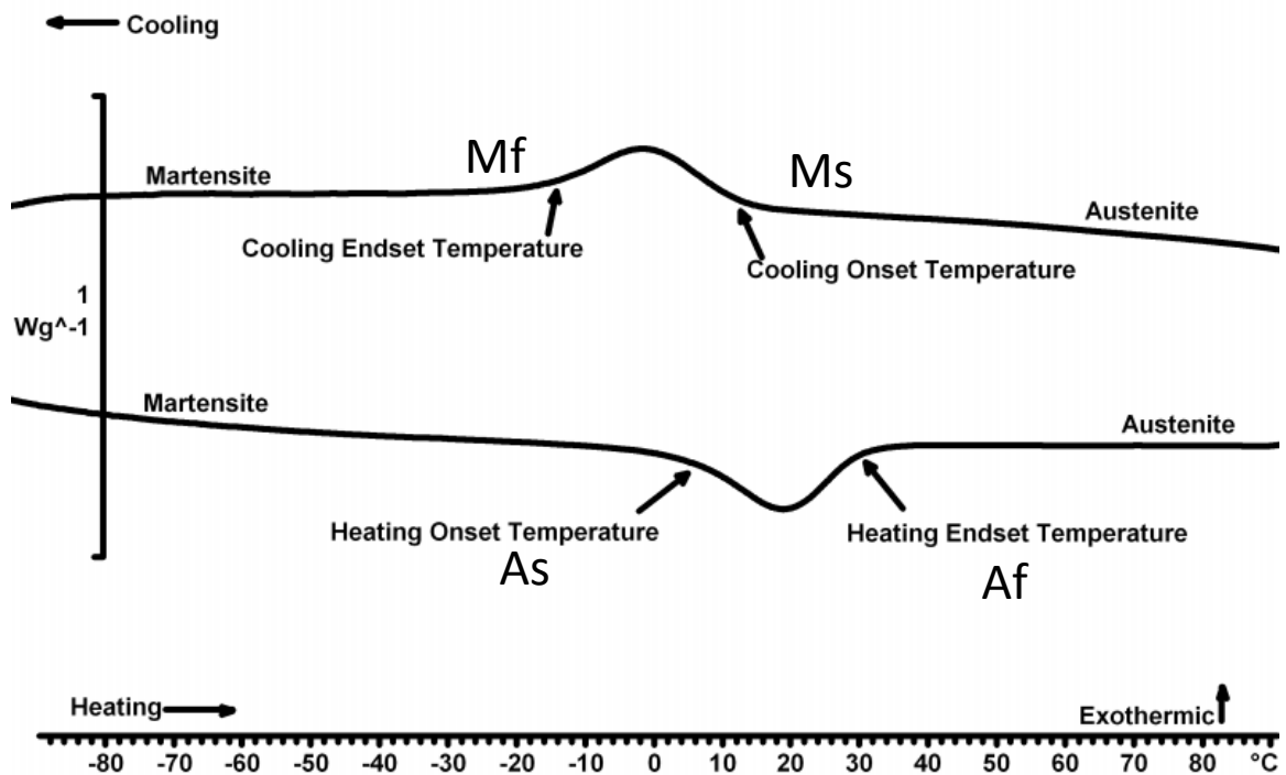
Figure 1: Example of DSC Thermogram
