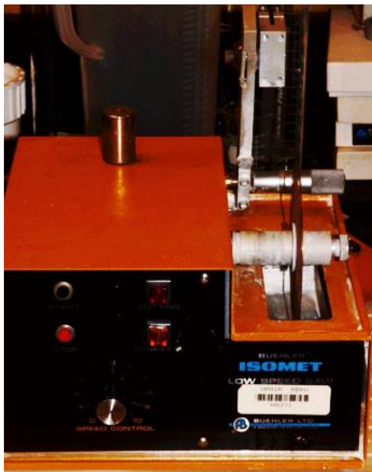
Figure 2: Isomet Diamond Saw used to section wires
