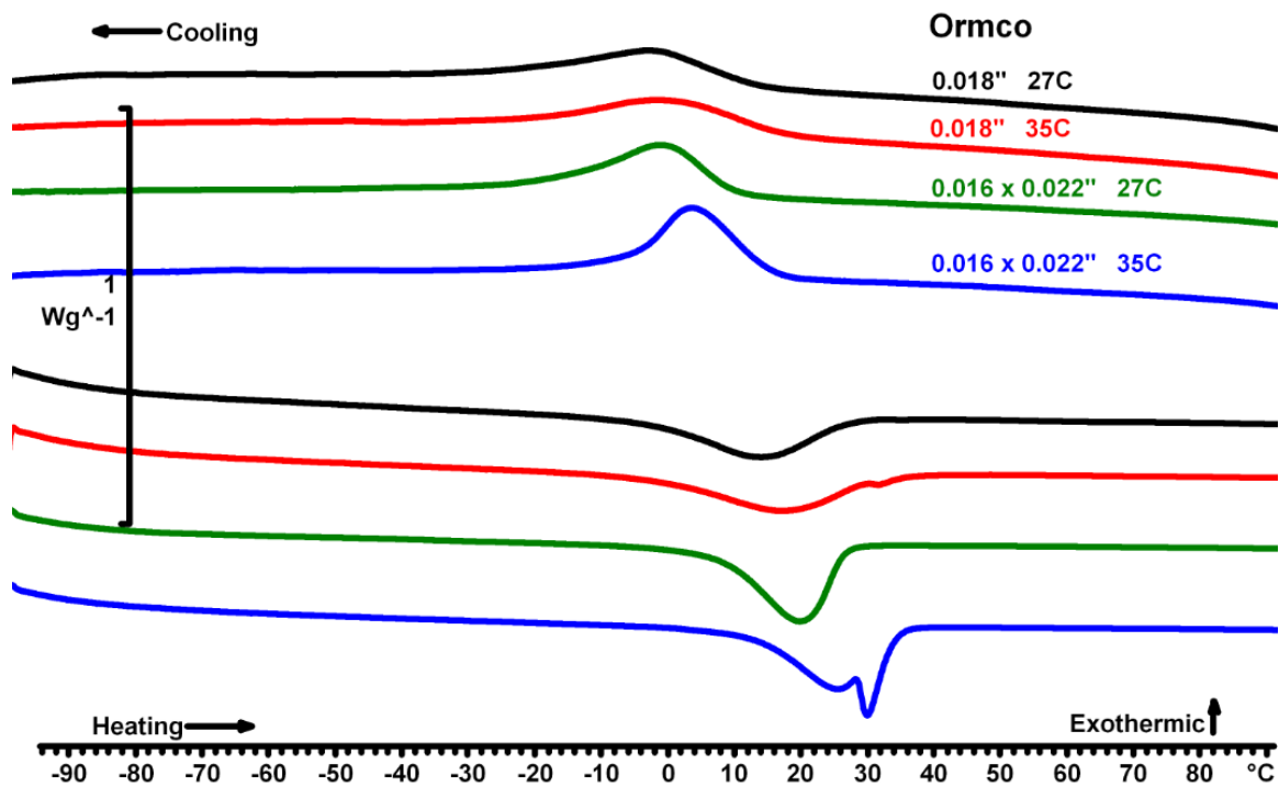
Figure 13: Thermogram for all variants of Ormco CuNiTi wires
