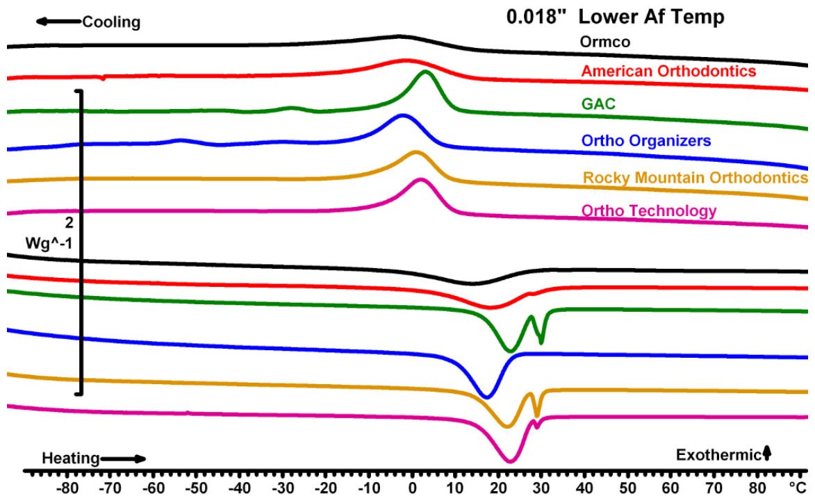
Figure 8: Thermogram for 0.018" wires with Af of 27°C
