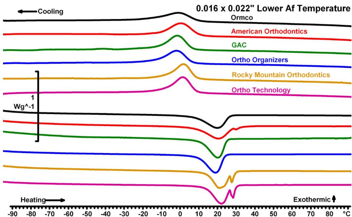
Figure 9: Thermogram for 0.016 x 0.022" wires with Af of 27°C
