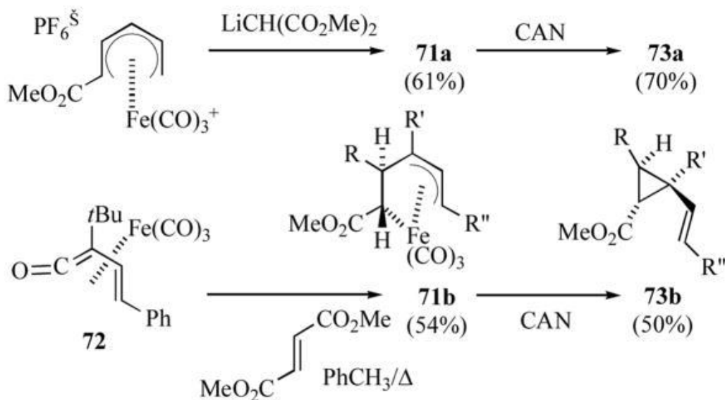
Scheme 12 Synthesis of vinylcyclopropanes via oxidative decomplexation of (3-pentene-1,5-diyl)iron complexes ( a , R = CH(CO 2 Me) 2 , R' = R'' = H; b , R = CO 2 Me, R' = tBu, R'' = Ph).
