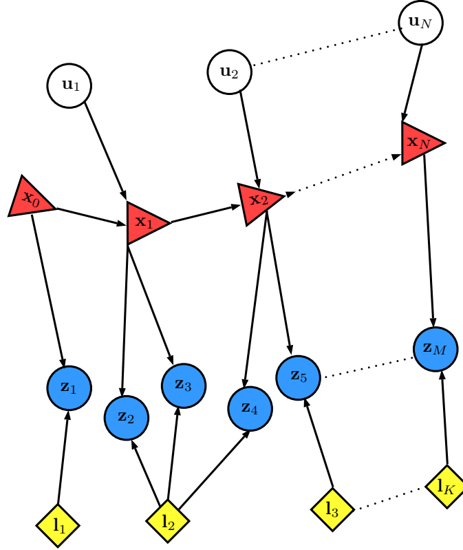
FIGURE 2.1: The belief network showing the cause-effect relationship of a robot navigation scenario. The robot (red) is given action inputs (plain) to navigate and collect landmark (yellow) measurements (blue). Same landmarks detected at multiple observations from a single pose indicates duplication which will be solved by data association.
