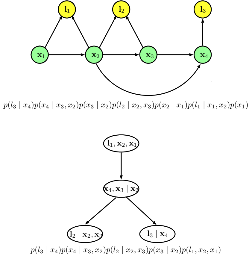
FIGURE 3.1: Bayes network and Bayes tree representations of the factor graph example used in last chapter with the elimination order O = [l_3, l_2, l_1, x_4, x_3, x_2, x_1] . The factorization of the factor graph joint probability density is mentioned for both the representations.
