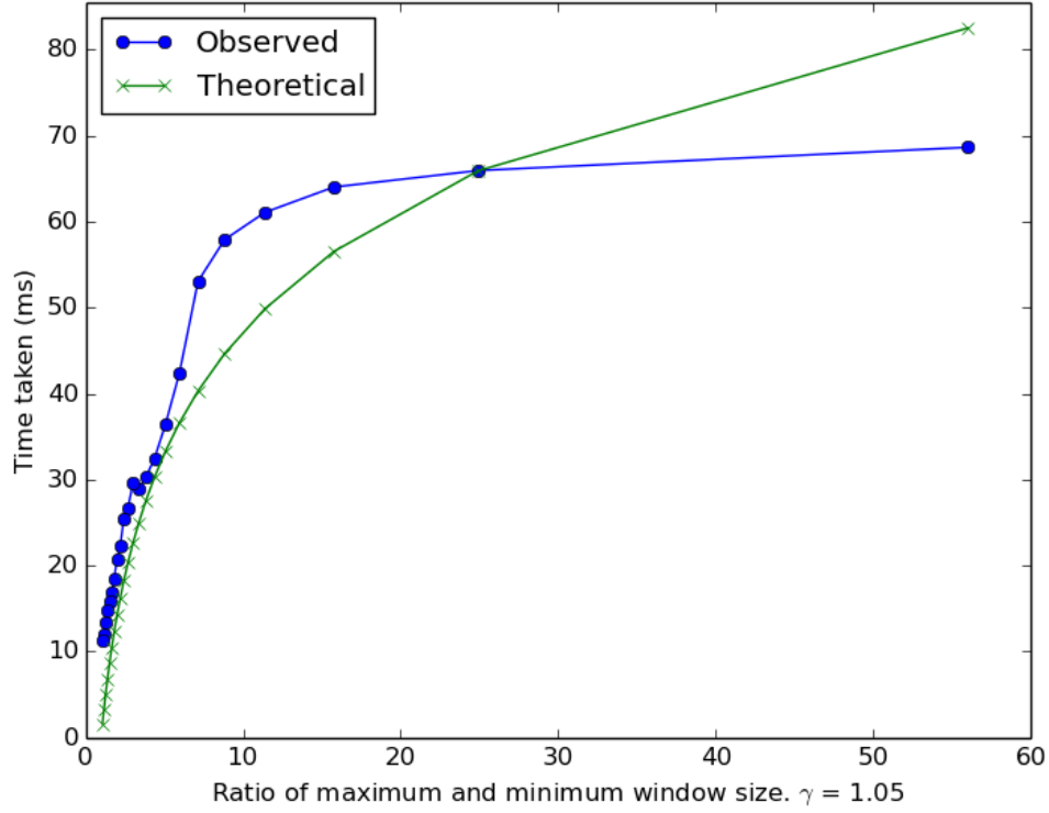
FIGURE 5.1: Comparison of ratio of maximum and minimum search window size with time taken for detection. It is clear from the shape of curve (blue) connecting the time taken for every search size that it varies logarithmically. The ideal curve (green) is just shown as a reference of a log curve and is not metrically accurate because we are trying to explain the theoretical complexity.
