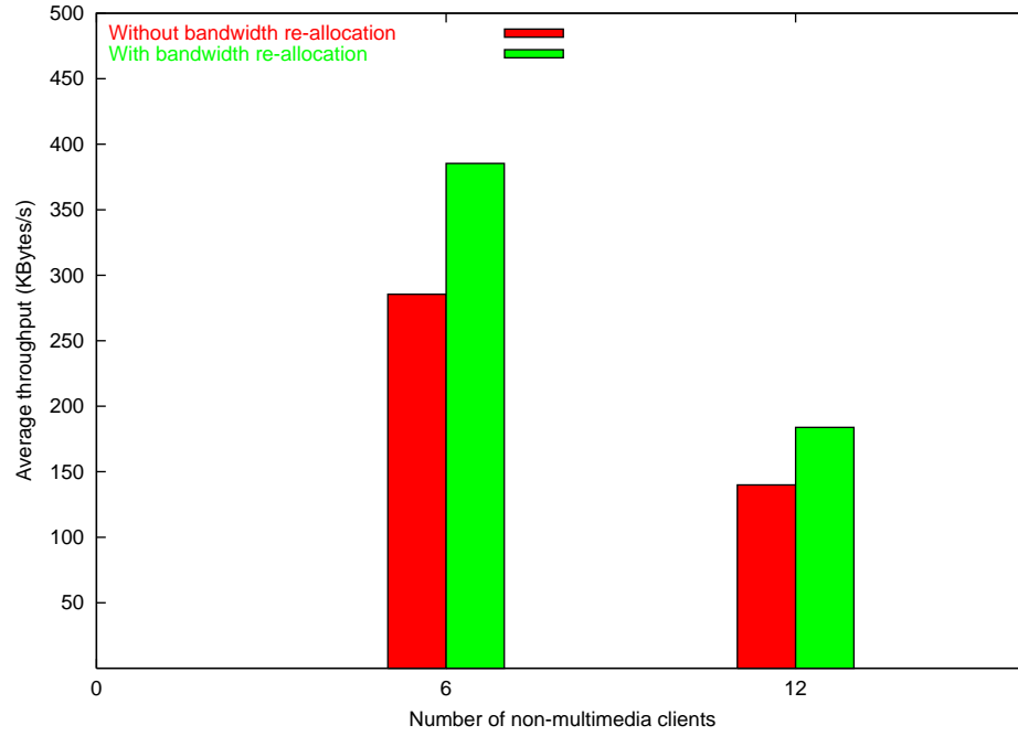
Figure 5.21: Average throughput with and without bandwidth re-allocation policies under Clarity when multimedia service class is under-utilized
