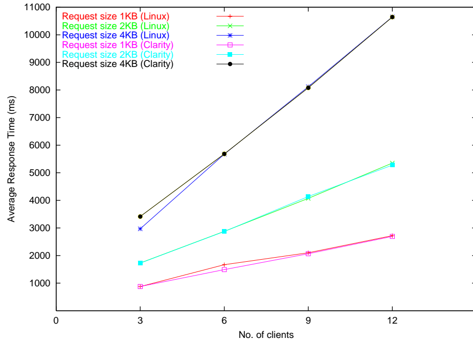
Figure 5.10: Performance comparison of Linux and Clarity in the presence of only non-multimedia clients: Average response time
