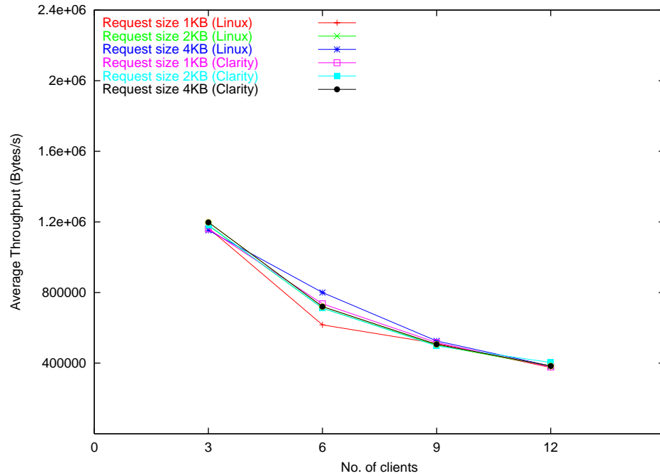
Figure 5.9: Performance comparison of Linux and Clarity in the presence of only non-multimedia clients: Average throughput
