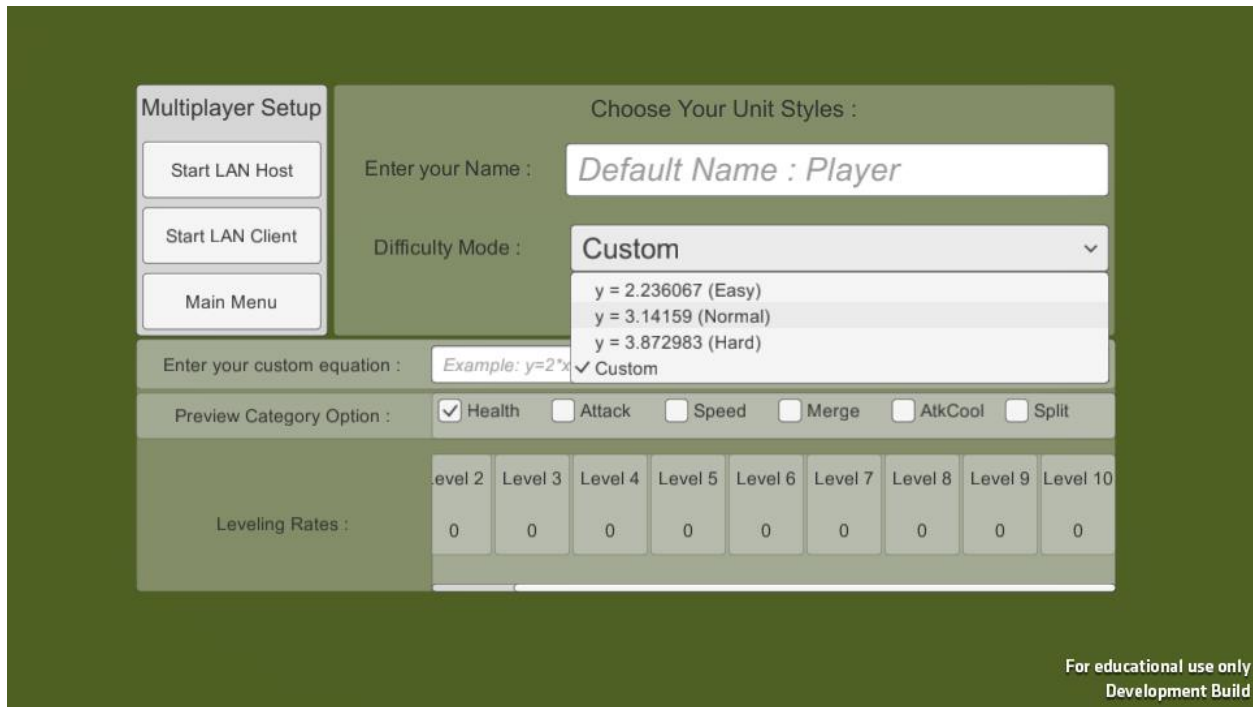
Figure 17: Multiplayer Mode in the Tool version, showing the LAN options, Attributes Editor and the Level Difficulty settings. The editor will only appear when the player chooses the “Custom” preset option.
