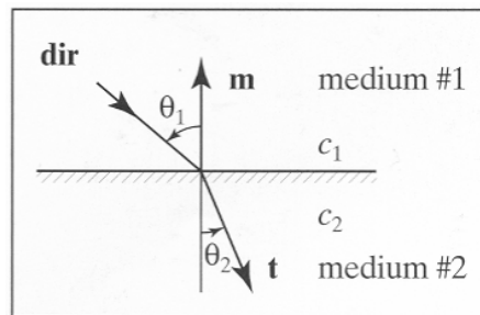
Figure 8: Light refracted as it leaves medium #1 and enters medium #2 [15].
