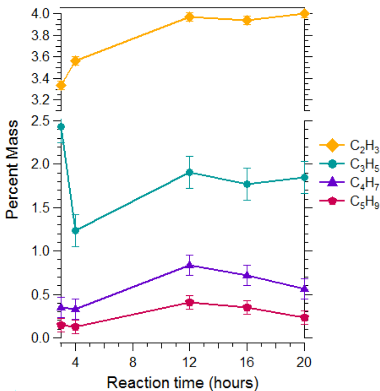
Figure 43. Mass Composition of mass spectrometry olefin ions as a function of reaction time. The mass composition is the percentage of the ions mass out of the total mass of all the organic ions, excluding the CO and CO 2 ions and the HO family ions. Ions plotted are (from top to bottom): C 2 H 3 (yellow, diamond), C 3 H 5 (blue, circle), C 4 H 7 (purple, triangle), and C 5 H 9 (violet, pentagon).
