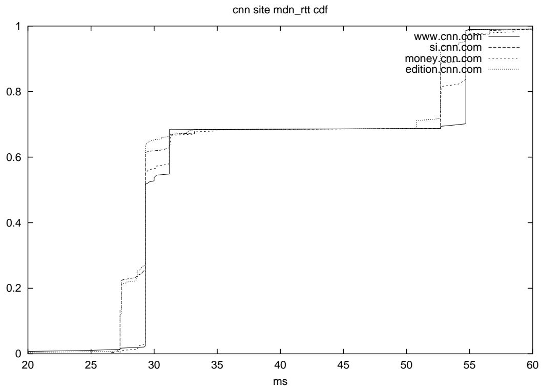
Figure 4.6: CDF of Median RTTs of CNN Cluster
