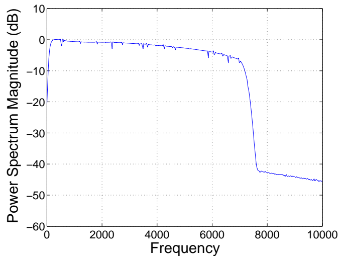
Figure 5.9: PSD of linear frequency sweep with “spatial” setting off.
