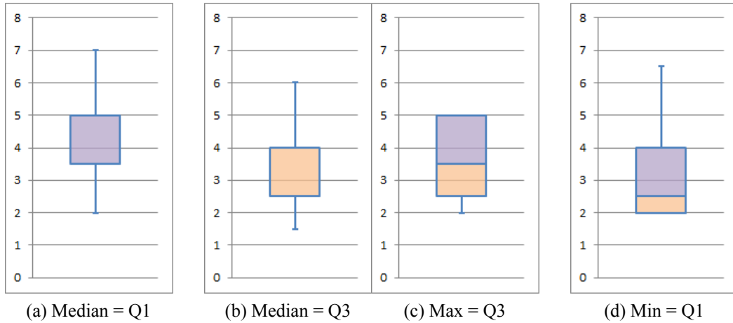
Figure F.2: Squished box plots
