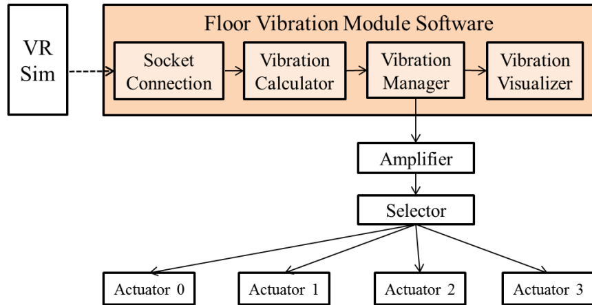
Figure 12: Floor Vibration Module Software Architecture
