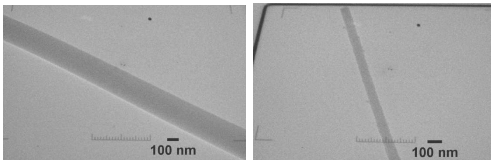
FIGURE 19: TEM IMAGES SHOWING SOLID NANORODS FORMED IN COMMERCIAL (LEFT) AND HOMEMADE (RIGHT) AAO TEMPLATES. DIAMETERS CORRESPOND WELL WITH THE TEMPLATE PORE SIZES.
