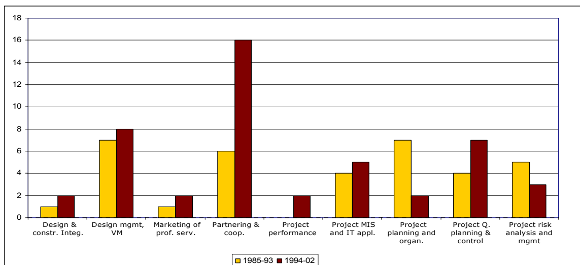
Figure 4-12. Project management
