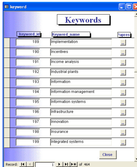
Figure 4-9. Keywords screen
