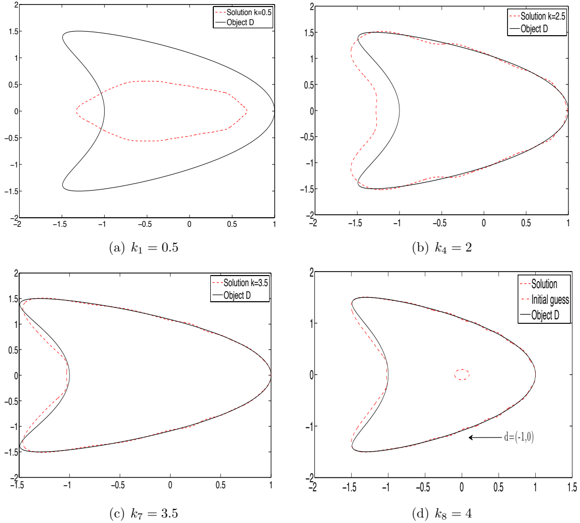
Figure 4.8: Solution of the inverse scattering problem for the Kite using the multi-frequency method. The incident plane waves have fixed incidence direction d = (-1, 0) and varying wavenumbers k_j = 0.5j , where j = 1, \dots, 8 . We use as the initial guess for the multi-frequency the circle with center at the origin and radius 0.1. The solution space with trigonometric polynomials of degree N_r = 20 is used for the method. We have the partial solution obtained at the wavenumber: (a) k_1 = 0.5 , (b) k_4 = 2 , and (c) k_7 = 3.5 . In (d), we have the solution using all frequencies.
