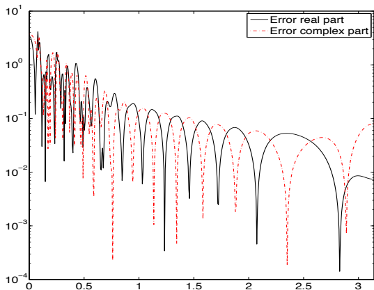
(c) Absolute errors for k = 6
