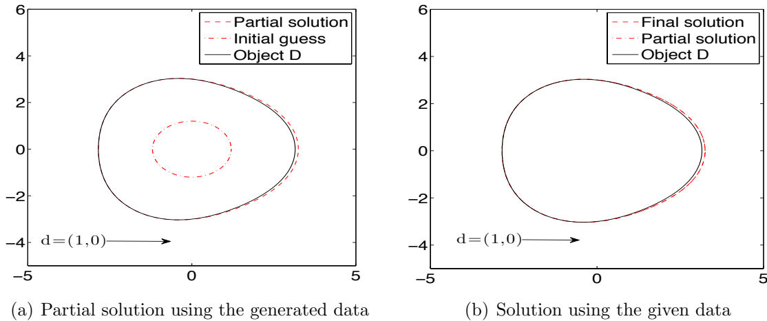
Figure 5.15: We use the RLA-C method to solve the inverse problem for the Egg. We have the far field pattern at the points \hat{x}_l = (2l - 1)\pi/N_{ff} , for l = 1, \dots, N_{ff} , with N_{ff} = 32 , generated by the scattering of two incident plane waves with incidence direction d = (1, 0) and wavenumbers k_a = 55 and k_b = 56 . We generate far field data for wavenumbers k_m = m , for m = 1, \dots, 54 . We use the parameter \epsilon_{\hat{x}} = \pi/2 to decide the generated far field pattern that we use for Method C. The initial guess x^{(0)} for the RLA-C method is the circle with center at the origin and radius 1.2. In (a) we present the result obtained applying Method C to the generated data, the object D , and the initial guess used in the RLA-C method, and in (b) we present the result obtained using the RLA-C method, the object D , and the answer obtained using Method C.
