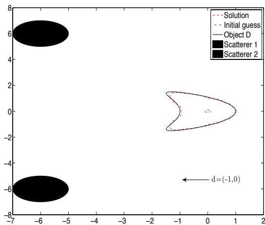
(a) k_j = 0.5j , N_r = 30 , N_{\text{inc}} = 8 , d = (-1, 0)
