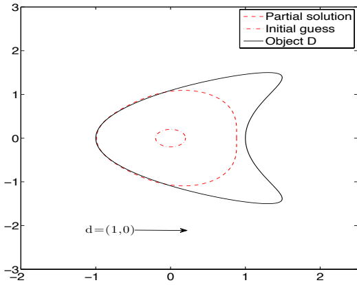
(a) Partial solution using the generated data
