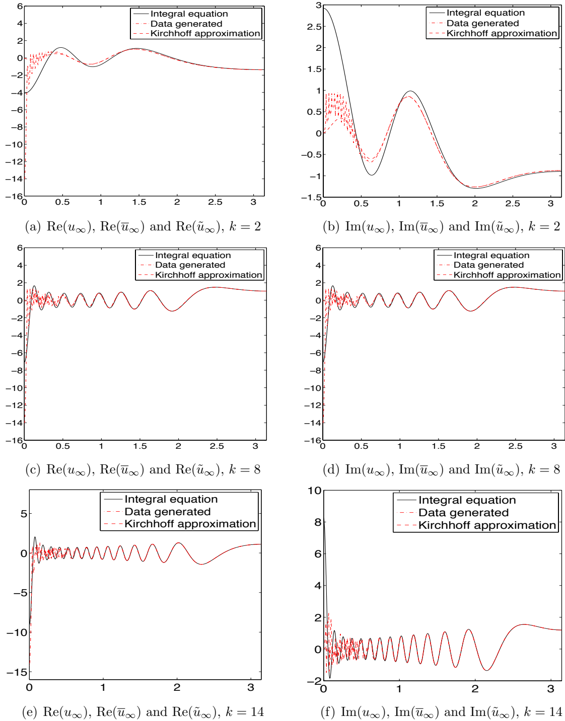
Figure 5.5: Comparison of the far field pattern obtained for the ellipse with k_a = 19 and k_b = 20 and d = (1, 0) by the Nyström method, labeled here as the Integral Equation, by the Kirchhoff approximation and by the our data generating procedure. In (a), (c) and (e) we have the real part of the far field patterns \text{Re}(u_\infty) , \text{Re}(\bar{u}_\infty) and \text{Re}(\tilde{u}_\infty) , where black is used for the Nyström method, \text{Re}(u_\infty) , the red pattern ‘-.’ for the data generating procedure, \text{Re}(\bar{u}_\infty) , and the red pattern ‘-’ is used for the Kirchhoff approximation, \text{Re}(\tilde{u}_\infty) , respectively for k = 2 , k = 8 and k = 14 . In (b), (d) and (f) we have the real part of \text{Re}(u_\infty) , \text{Re}(\bar{u}_\infty) and \text{Re}(\tilde{u}_\infty) , where black is used for the Nyström method, \text{Re}(u_\infty) , the red pattern ‘-.’ for the data generating procedure \text{Re}(\bar{u}_\infty) , and the red pattern ‘-’ is used for the Kirchhoff approximation, \text{Re}(\tilde{u}_\infty) , respectively for k = 2 , k = 8 and k = 14 .
