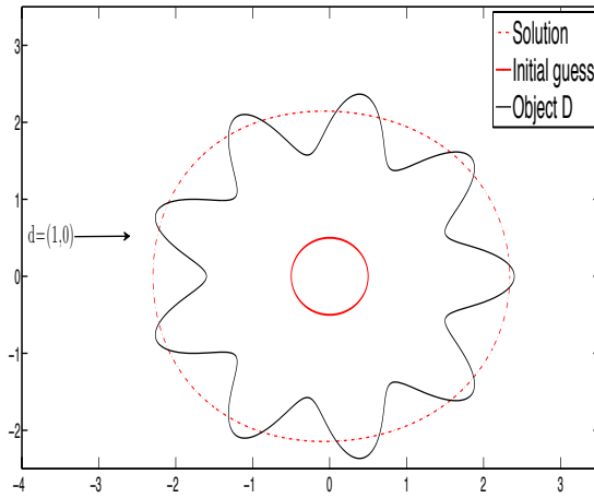
(c) k = 0.5 , N_r = 8 , d = (1, 0)
