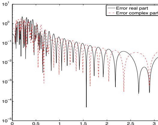
(f) Relative errors for k = 10
