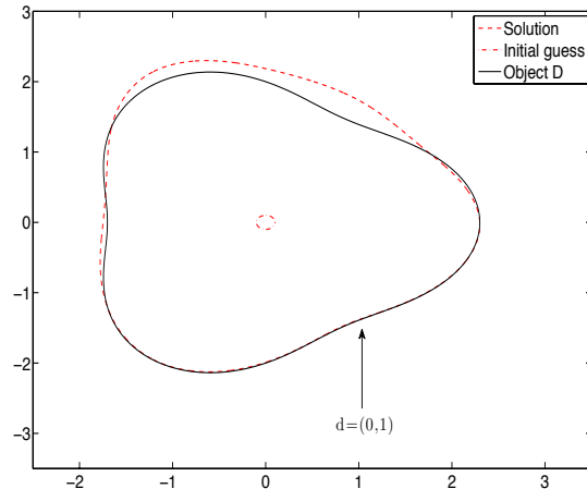
(b) Spline, k = 1 , d = (0, 1) , N_r^2 = 12
