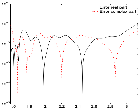
(e) Absolute errors for k = 12
