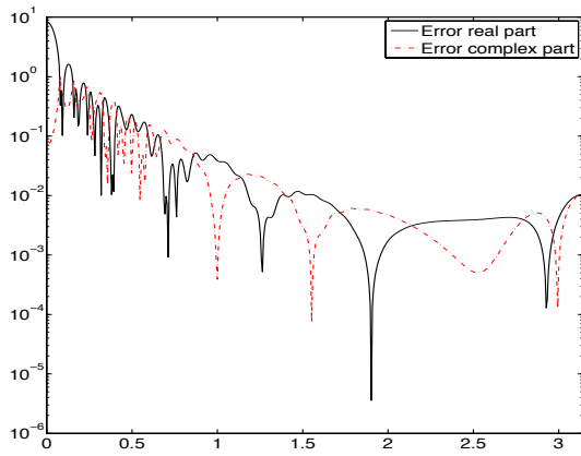
(a) Absolute errors for k = 2
