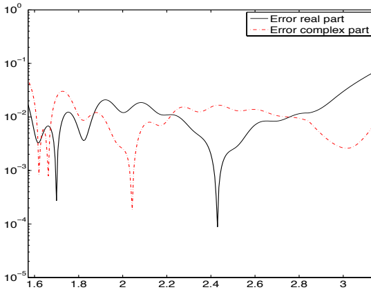
(c) Absolute errors for k = 7
