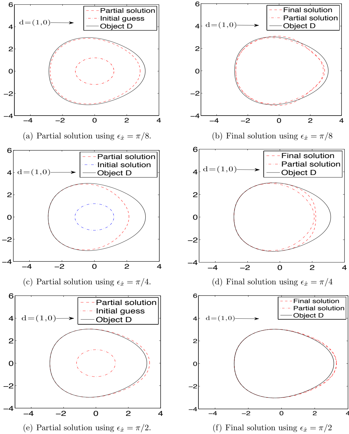
Figure 5.17: We use the RLA-C method to solve the inverse problem for the Egg. We have the far field pattern at the points \hat{x}_l = (2l - 1)\pi/N_{ff} , for l = 1, \dots, N_{ff} , with N_{ff} = 32 , generated by the scattering of two incident plane waves with incidence direction d = (1, 0) and wavenumbers k_a = 40 and k_b = 41 . We generate far field data for wavenumbers k_m = m , for m = 1, \dots, 44 . We vary the parameter \epsilon_{\hat{x}} that we use to decide the generated far field pattern that we use for Method C. The initial guess x^{(0)} for the RLA-C method is the circle with center at the origin and radius 1.2. We have the result obtained applying Method C in the generated data, the object D , and the initial guess used in the RLA-C method for (a) \epsilon_{\hat{x}} = \pi/2 , (c) \epsilon_{\hat{x}} = \pi/4 , and (e) \epsilon_{\hat{x}} = \pi/8 , and we have the result obtained after using the RLA-C method, the object D , and the answer obtained using Method C for (b) \epsilon_{\hat{x}} = \pi/2 , (d) \epsilon_{\hat{x}} = \pi/4 , and (f) \epsilon_{\hat{x}} = \pi/8 .
