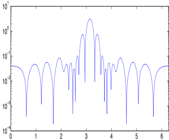
(c) Difference of \text{Re}(u_\infty) for Nyström and Kirchoff
