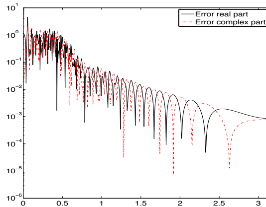
(f) Relative errors for k = 14
