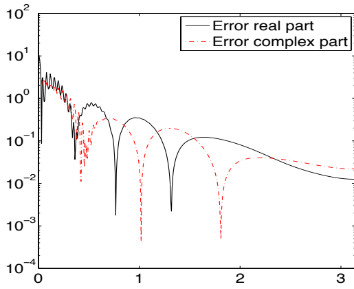
(a) Absolute errors for k = 2
