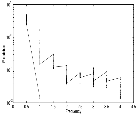
(a) Kite, k_j = 0.5j , j = 1, \dots, 8 , d = (-1, 0)
