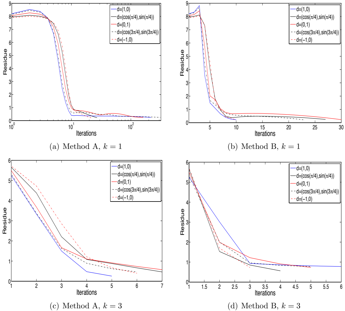
Figure 4.3: Plot of residue versus number of iterations for all the scenarios of this example. Each curve represents the residue in each iteration for the problem using an incident plane wave with wavenumber k and incidence direction d using Method A or Method B. (a) Method A with k = 1 . (Note here that the x -axis is on the log-scale for only this figure.) (b) Method B with k = 1 . (c) Method A with k = 3 . (d) Method B with k = 3 .
