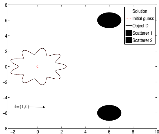
(c) k_j = 0.5j , N_r = 10 , N_{\text{inc}} = 12 , d = (1, 0)
