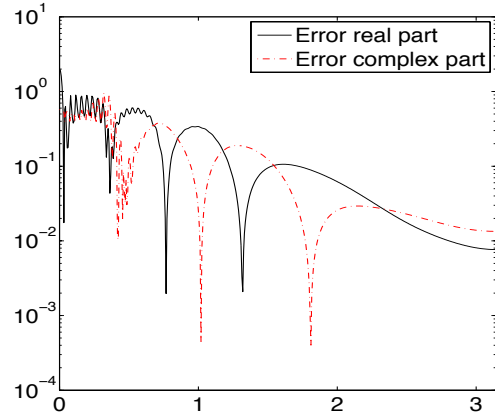
(b) Relative errors for k = 2
