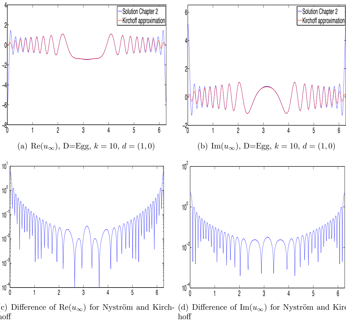
Figure 5.2: Comparison of the far field pattern obtained for the Egg with k = 10 and d = (1, 0) by the Nyström method and by the Kirchhoff approximation. In (a) and (b) we have respectively the real and imaginary parts of the far field pattern, where blue is used for the Nyström method and red for the Kirchhoff approximation. In (c) and (d) we have respectively the absolute value of the difference between the real and imaginary parts of the solutions given by the Nyström method and the Kirchhoff approximation. Note that we have a log scale on the y -axis of the graphs.
