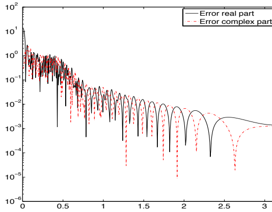
(e) Absolute errors for k = 14
