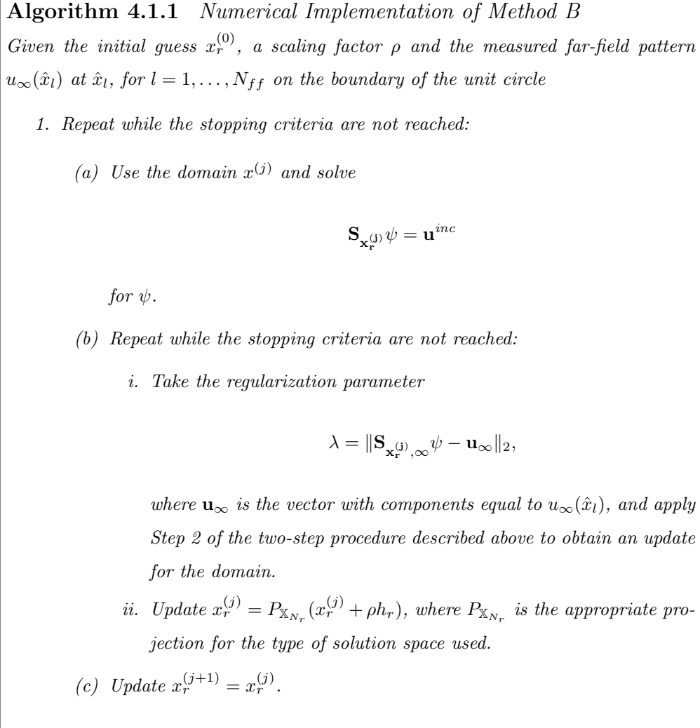
Figure 4.2: Implementation of Method B described in Chapter 2 for solving the inverse problem for an object D with Dirichlet boundary conditions using single frequency far field pattern measures.
