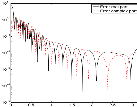
(c) Absolute errors for k = 6
