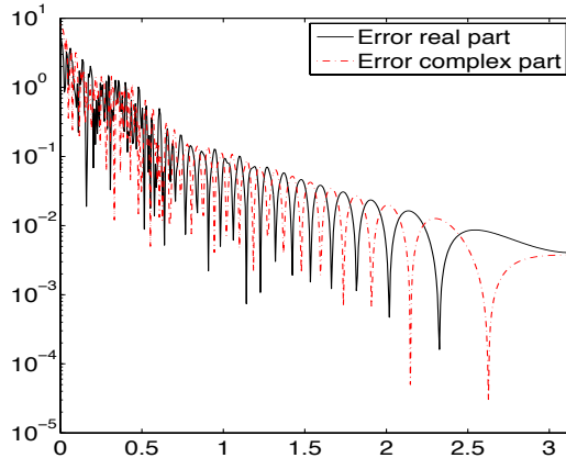
(e) Absolute errors for k = 14
