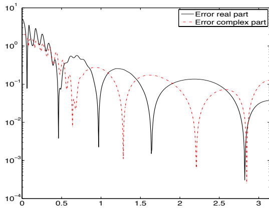
(a) Absolute errors for k = 2
