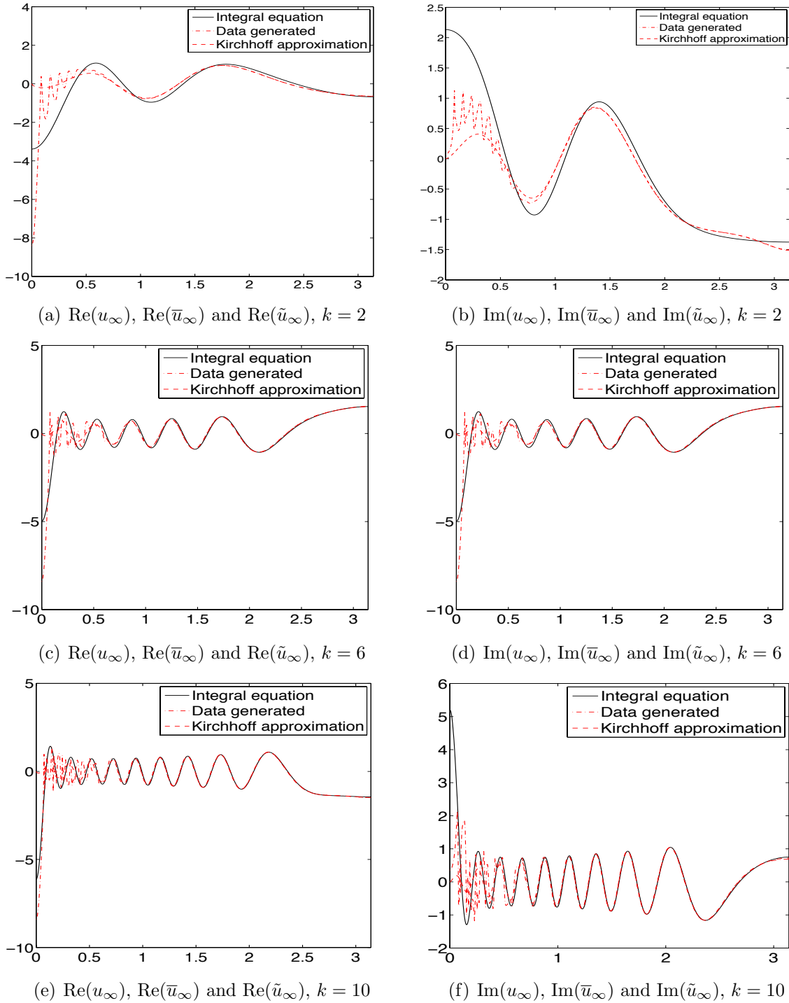
Figure 5.8: Comparison of the far field pattern obtained for the Egg with k_a = 11 and k_b = 12 and d = (1,0) by the Nyström method, labeled here as the Integral Equation, by the Kirchhoff approximation and by the our data generating procedure. In (a), (c) and (e) we have the real part of the far field patterns \text{Re}(u_\infty) , \text{Re}(\bar{u}_\infty) and \text{Re}(\tilde{u}_\infty) , where black is used for the Nyström method, \text{Re}(u_\infty) , the red pattern ‘-.’ for the data generating procedure, \text{Re}(\bar{u}_\infty) , and the red pattern ‘-’ is used for the Kirchhoff approximation, \text{Re}(\tilde{u}_\infty) , respectively for k = 2 , k = 6 and k = 10 . In (b), (d) and (f) we have the real part of \text{Re}(u_\infty) , \text{Re}(\bar{u}_\infty) and \text{Re}(\tilde{u}_\infty) , where black is used for the Nyström method, \text{Re}(u_\infty) , the red pattern ‘-.’ for the data generating procedure \text{Re}(\bar{u}_\infty) , and the red pattern ‘-’ is used for the Kirchhoff approximation, \text{Re}(\tilde{u}_\infty) , respectively for k = 2 , k = 6 and k = 10 .
