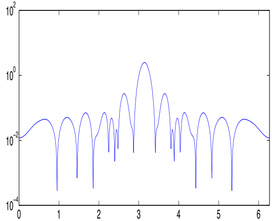
(d) Difference of \text{Im}(u_\infty) for Nyström and Kirchoff
