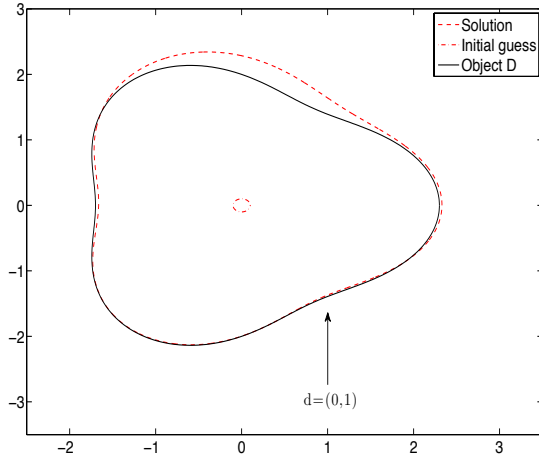
(a) Trigonometric, k = 1 , d = (0, 1) , N_r^1 = 5
