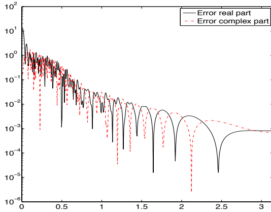
(c) Absolute errors for k = 8
