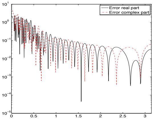
(e) Absolute errors for k = 10
