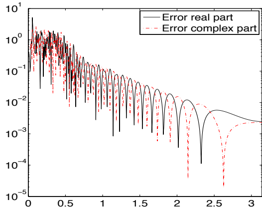
(f) Relative errors for k = 14
