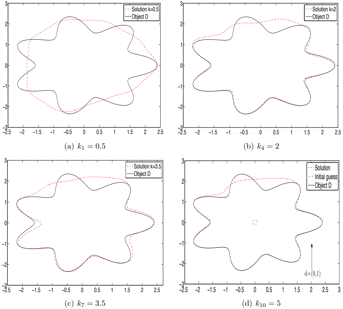
Figure 4.9: Solution of the inverse scattering problem for the 7-gear using the multi-frequency method. The incident plane waves have fixed incidence direction d = (0, 1) and varying wavenumbers k_j = 0.5j , where j = 1, \dots, 10 . We use as the initial guess for the multi-frequency the circle with center at the origin and radius 0.1. The solution space with trigonometric polynomials of degree N_r = 10 is used for the method. We have the partial solution obtained at the wavenumber: (a) k_1 = 0.5 , (b) k_4 = 2 , and (c) k_7 = 3.5 . In (d), we have the solution using all frequencies.
