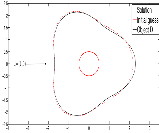
(a) k = 0.5 , N_r = 5 , d = (1, 0)
