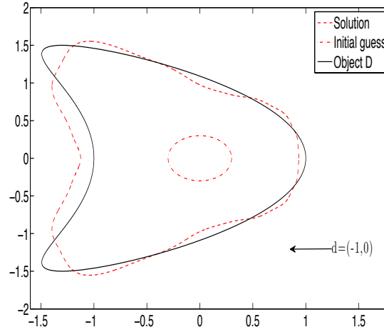
(f) Spline, k = 1 , d = (-1, 0) , N_r^2 = 40
