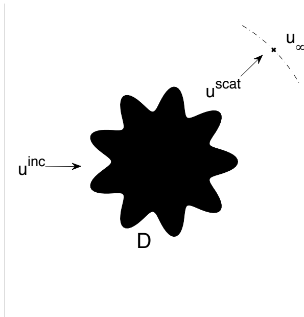
Figure 2.1: The direct scattering problem of finding the field scattered by an impenetrable obstacle.
