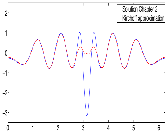
(a) \text{Re}(u_\infty) , D=\text{Kite} , k = 20 , d = (-1, 0)
