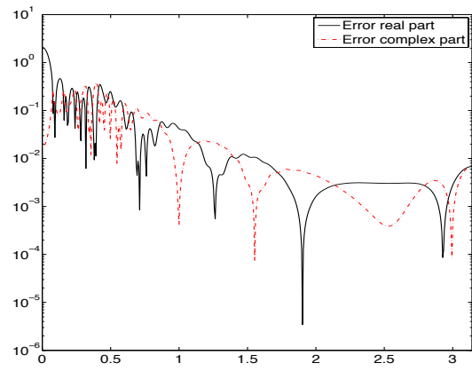
(b) Relative errors for k = 2
