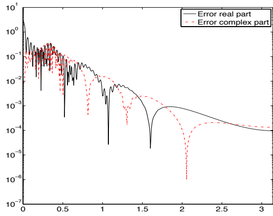
(b) Relative errors for k = 2
