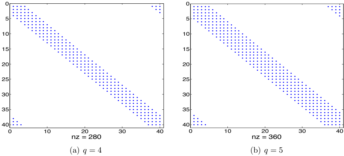
Figure 4.1: Matrix \mathbf{I}^1 for a fixed number of coefficients N_r = 40 and varying order q . (a) q = 4 . (b) q = 5 . Each dot represents a nonzero element, and where there are no dots, the matrix entries are filled by zeros.
