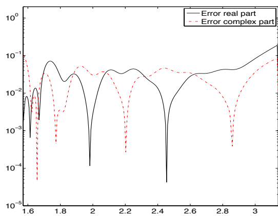
(f) Relative errors for k = 12
