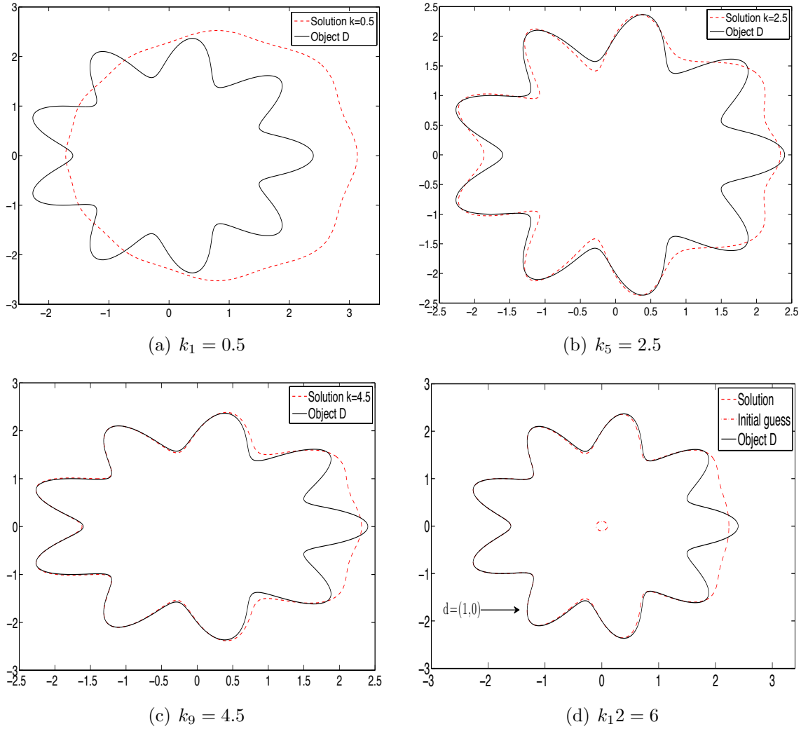
Figure 4.10: Solution of the inverse scattering problem for the 9-gear using the multi-frequency method. The incident plane waves have fixed incidence direction d = (1, 0) and varying wavenumbers k_j = 0.5j , where j = 1, \dots, 12 . We use as the initial guess for the multi-frequency the circle with center at the origin and radius 0.1. The solution space with trigonometric polynomials of degree N_r = 10 is used for the method. We have the partial solution obtained at the wavenumber: (a) k_1 = 0.5 , (b) k_5 = 2.5 , and (c) k_9 = 4.5 . In (d), we have the solution using all frequencies.
