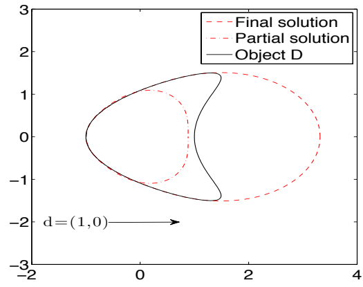
(b) Solution using the given data
