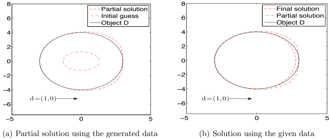
Figure 5.14: We use the RLA-C method to solve the inverse problem for the ellipse with parameterization x(t) = (3 \cos(t), 4 \sin(t)) . We have the far field pattern at the points \hat{x}_l = (2l - 1)\pi/N_{ff} , for l = 1, \dots, N_{ff} , with N_{ff} = 32 , generated by the scattering of two incident plane waves with incidence direction d = (1, 0) and wavenumbers k_a = 50 and k_b = 51 . We generate far field data for wavenumbers k_m = m , for m = 1, \dots, 49 . We use the parameter \epsilon_{\hat{x}} = \pi/2 to decide the generated far field pattern that we use for Method C. The initial guess x^{(0)} for the RLA-C method is the circle with center at the origin and radius 1.3. In (a) we present the result obtained applying Method C to the generated data, the object D , and the initial guess used in the RLA-C method, and in (b) we present the result obtained using the RLA-C method, the object D , and the answer obtained using Method C.
