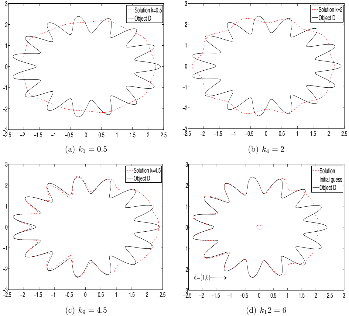
Figure 4.11: Solution of the inverse scattering problem for the 15-gear using the multi-frequency method. The incident plane waves have fixed incidence direction d = (1, 0) and varying wavenumbers k_j = 0.5j , where j = 1, \dots, 12 . We use as the initial guess for the multi-frequency the circle with center at the origin and radius 0.1. The solution space with trigonometric polynomials of degree N_r = 17 is used for the method. We have the partial solution obtained at the wavenumber: (a) k_1 = 0.5 , (b) k_4 = 2 , and (c) k_9 = 4.5 . In (d), we have the solution using all frequencies.
