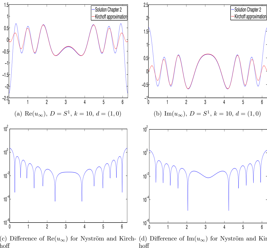
Figure 5.1: Comparison of the far field pattern obtained for the circle S^1 with k = 10 and d = (1, 0) by the Nyström method and by the Kirchhoff approximation. In (a) and (b) we have respectively the real and imaginary parts of the far field pattern, where blue is used for the Nyström method and red for the Kirchhoff approximation. In (c) and (d) we have respectively the absolute value of the difference between the real and imaginary parts of the solutions given by the Nyström method and the Kirchhoff approximation. Note that we have a log scale on the y -axis of the graphs.
