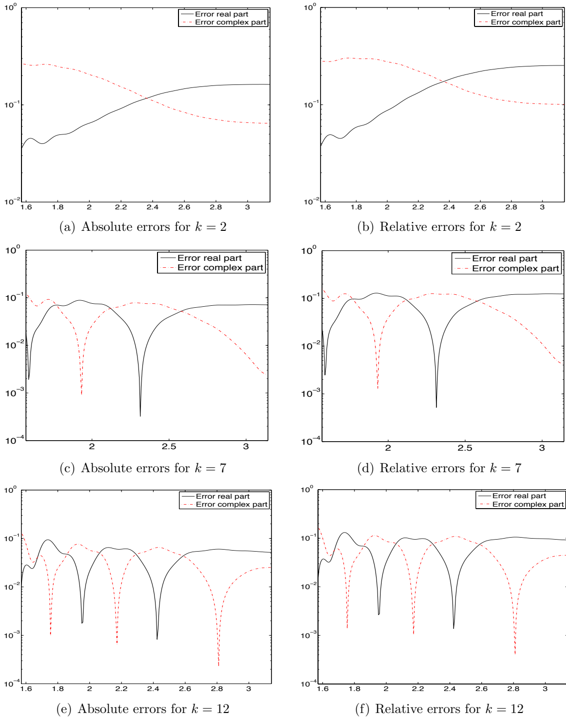
Figure 5.12: Absolute and relative error with respect to the far field obtained with the Nyström method of the data generating procedure for the rotated Kite using k_a = 14 and k_b = 15 . We have the absolute error for the real part in black and the imaginary part in the red pattern ‘-.’ respectively for the frequencies: (a) k = 2 , (c) k = 7 and (e) k = 12 . In the other figures, the relative error for the real part is in black and for the imaginary part in the red pattern ‘-.’, respectively for the frequencies: (b) k = 2 , (d) k = 7 and (f) k = 12 . Note that we have a log scale on the y -axis of those graphs. The domain of these figures go from \pi/2 to \pi since it is not possible to take the Kirchhoff approximation from 0 to \pi because the object is not convex for those values.
