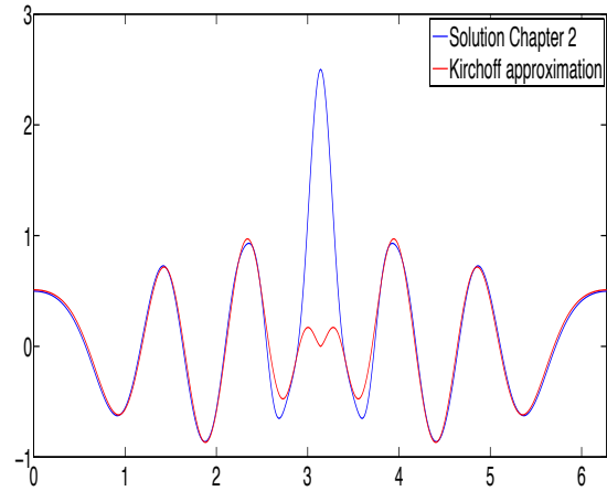
(b) \text{Im}(u_\infty) , D=\text{Kite} , k = 20 , d = (-1, 0)
