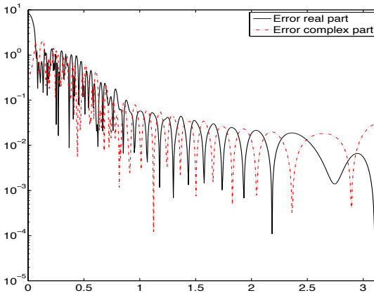
(e) Absolute errors for k = 10
