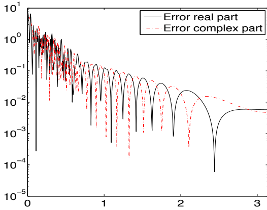
(c) Absolute errors for k = 8
