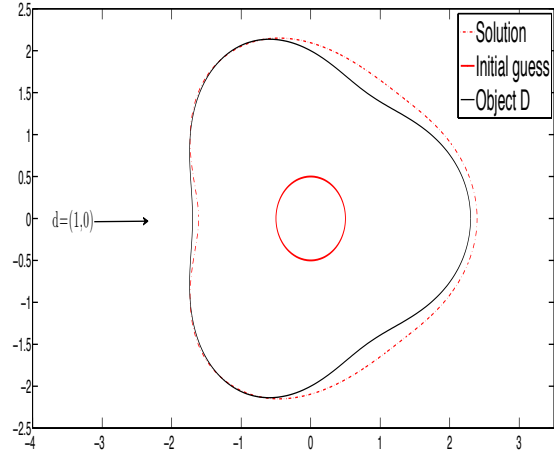
(b) k = 0.5 , N_r = 10 , d = (1, 0)
