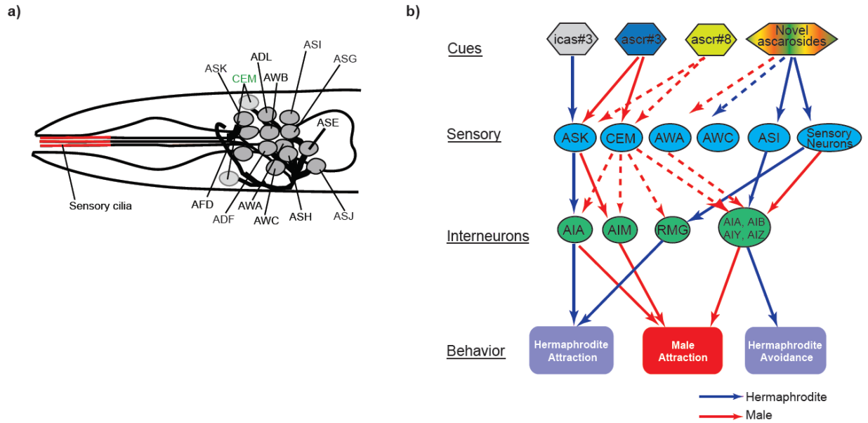
Fig. B3. Neural responses to C. elegans chemical mating signals. (A) Sensory neuroanatomy of C. elegans indicating different sensory neurons including the male-specific CEM neurons (green). Most of these sensory neurons have sensory cilia that extend to the tip of the nose, thereby sensing the environment. (B) Complex sensory transduction of ascarosides. Different derivatives are sensed by either core sensory neurons or sex-specific neurons. The red and blue lines indicate male signaling and hermaphrodite signaling respectively. The dotted red or blue line indicates a probable pathway that might be used to sense the signals.
