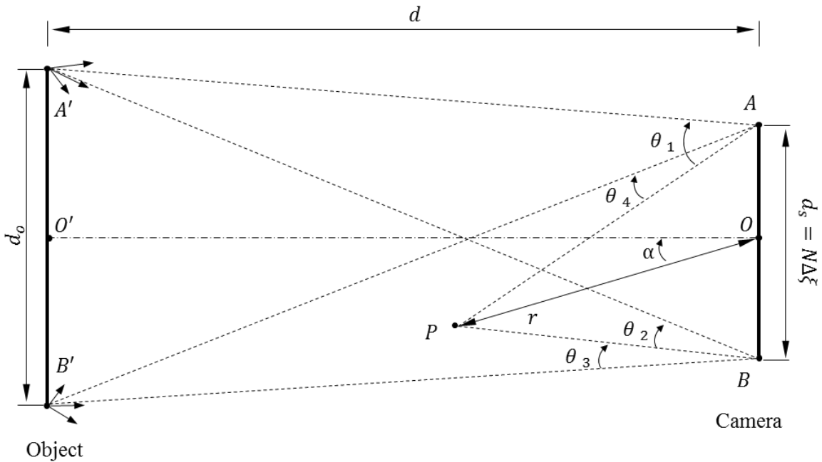
Fig. A.1. Geometrical setup of the optical system of the OH based on an enhanced lensless Fourier transform holographic setup. Indicated are geometrical major parameters defining the footprint of optical system.
