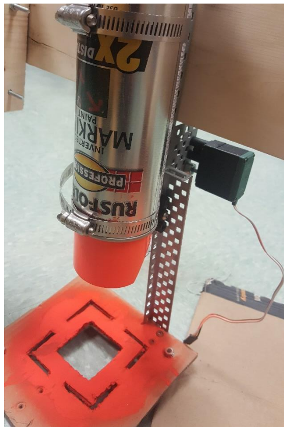
Figure 25 Sprayer and mask system
