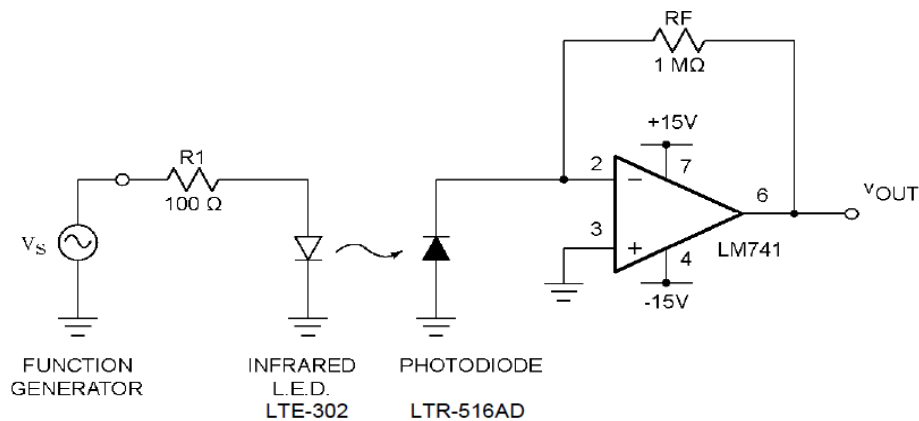
Figure 29: Example photodetector circuit to measure light intensity.
