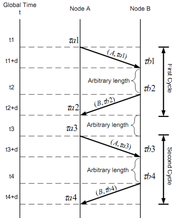
Equation 3: Time of flight calculation from PinPoint
