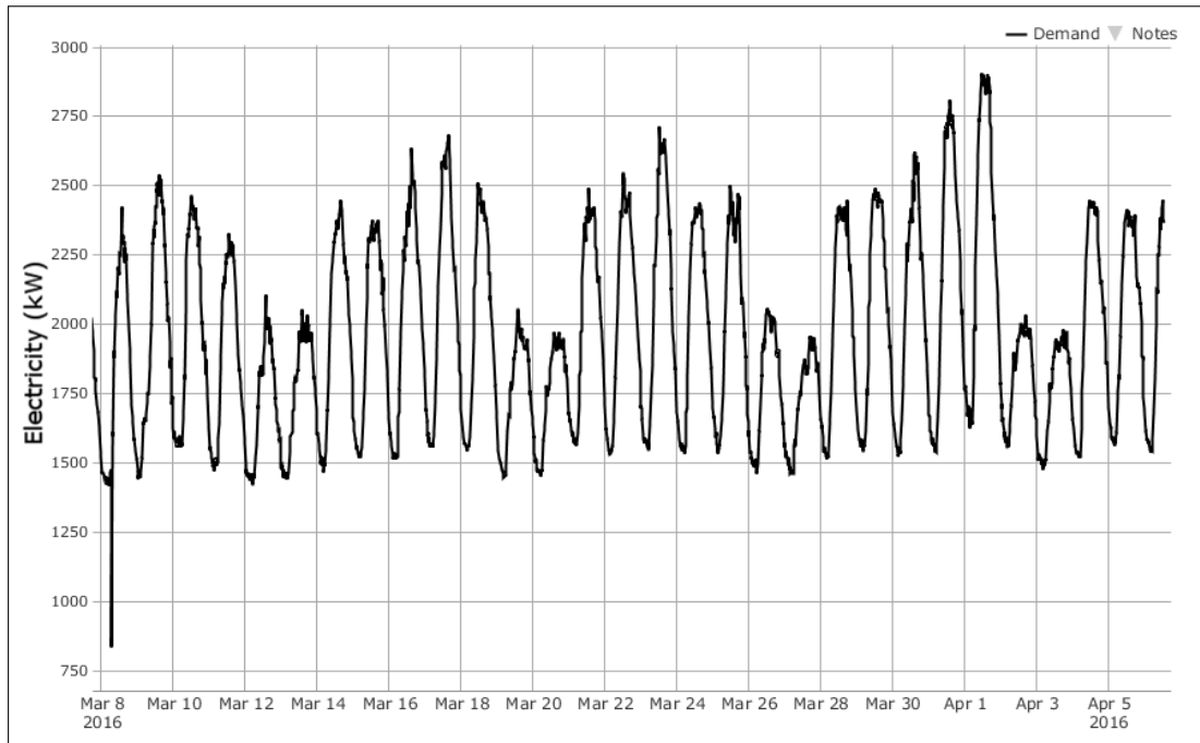
Figure 9: Example of a Building’s Power Consumption Over Time, from EDSM Data Accessed Through WebCtrl.
