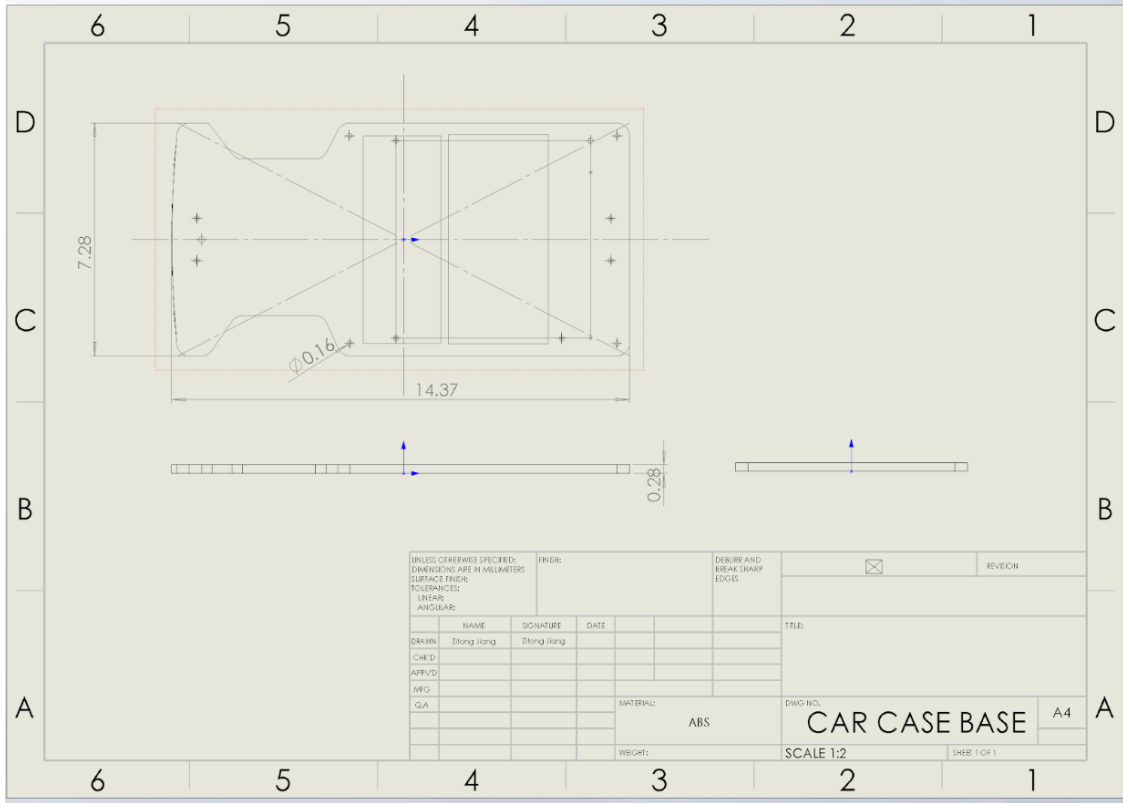
Figure 10: Car Case Base Design Drawing
