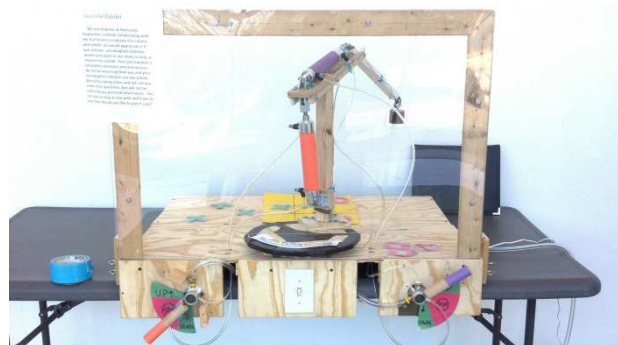
Figure 10 Color Coded Pistons, Handles Vertical
