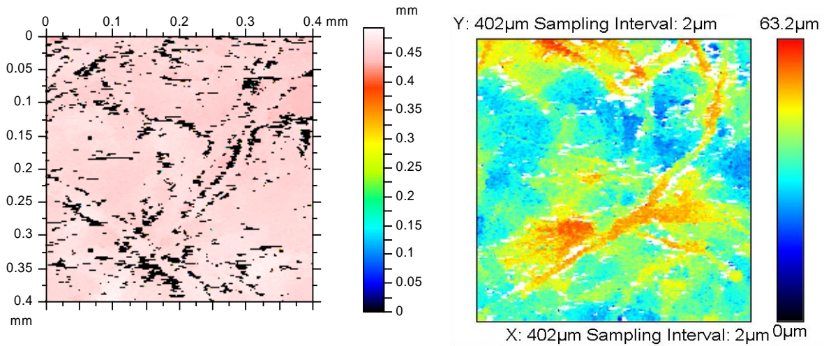
Figure 2: An example of a measurement of wood-stained paper before and after filtering
