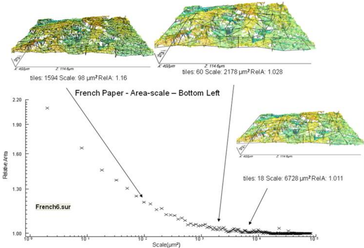
Figure 3: Area-scale analysis
