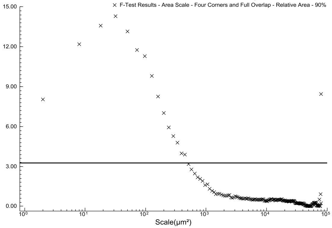
F-Test Results - Area Scale - Four Corners and Full Overlap - Relative Area - 90%
