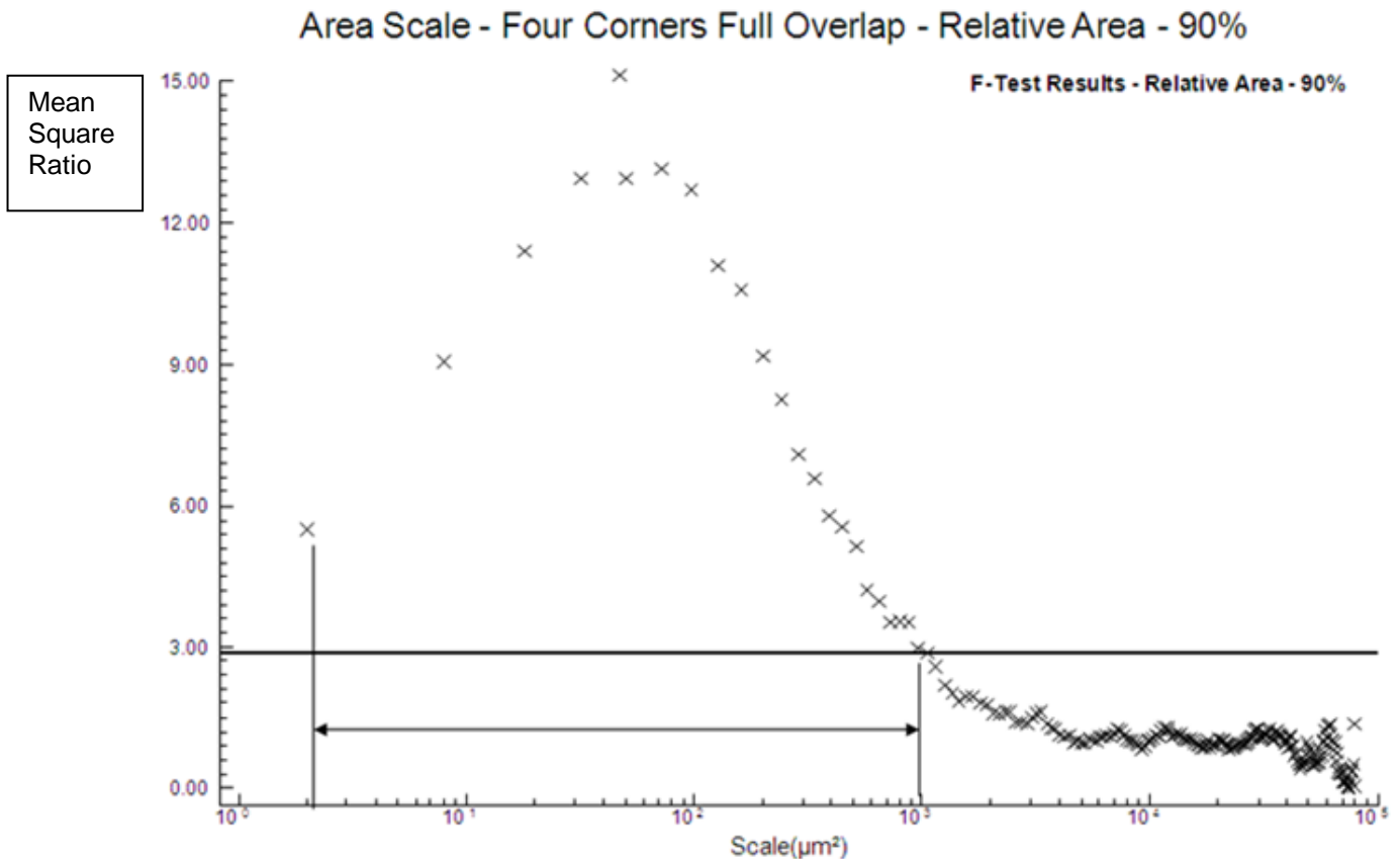
Figure 5: Scale based F-test of untreated a sample of French Paper versus wood-stained Paper
