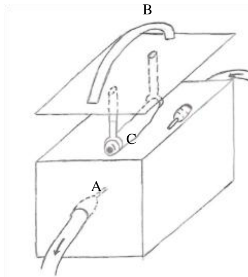
Figure 13: Original Lunchbox Design with syringe needles embedded in the walls (A), a handle on the top of the lid (B), and ring-shaped posts to hold the tissue (C).
