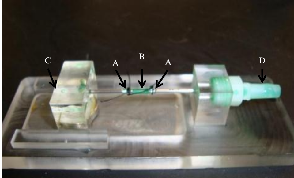
Figure 25: No leaking was observed around sutured tubing. In this image the sutures (A) and the silicone tubing (B) are shown. The inlet (D) and outlet (C) are also visible.
