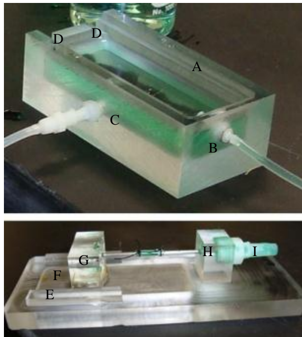
Figure 20: The components of the acrylic prototype chamber consist of a cut out for the placement of the lid (A), inlet female Luer connector (B), outlet male Luer connector (C), and two rectangular gaps for the track ridges to slide on (D). The components of the acrylic prototype lid consist of ridges for guidance of the moveable arm (E), an embedded steel track (F), a moveable arm (G), a stationary arm (H), and a male Luer connector for the wall connection (I).
