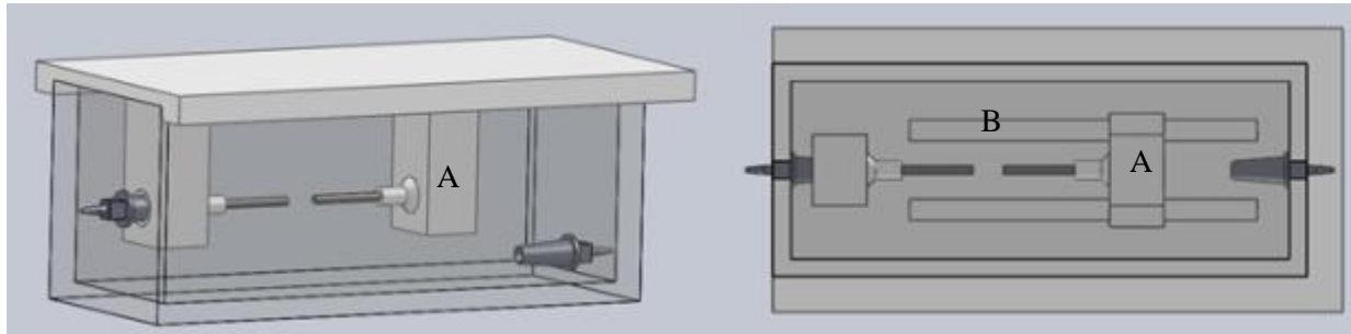
Figure 15: The first iteration of the sliding track design. A sliding T-shaped arm (A) moved along tracks (B) in order to adjust the positioning of one of the syringe needles.
