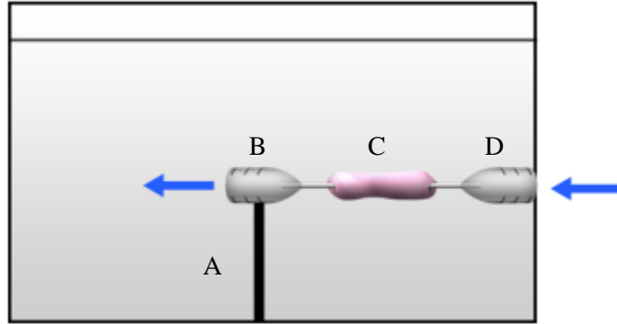
Figure 10: Open Cartridge Design 1 consists of a plastic arm (A) attached to the bottom face of the chamber. A syringe needle (B) is used to support the end of the tissue tube (C) while another syringe needle supports the other end at the inlet (D).
