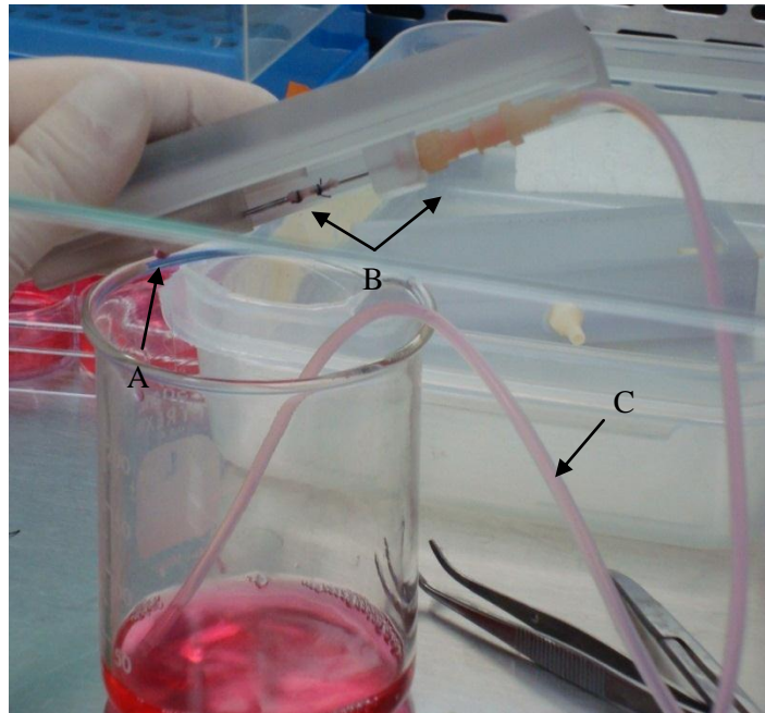
Figure 35: Media flows all the way through the tissue tube and comes out the end of the movable arm (A). No leaking is observed at the tissue-syringe interface or the Luer-tubing interface (B). Media flows from a beaker through the tubing and into the arms of the lid, priming the tubes in the process (C).
