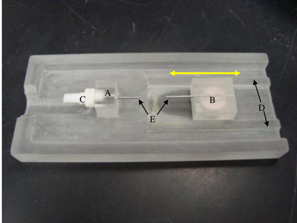
Figure 28: Lid of the final design, which includes the stationary arm (A), the movable arm (B), male Luer connector (C), the ridges for the magnetic track (D), and 18-gauge syringe tips (E). The movable arm's movement is illustrated by the yellow arrow.
