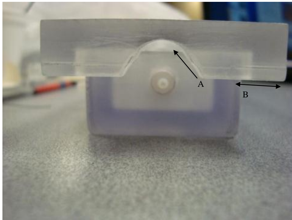
Figure 29: Arc cutout of the lid that enables gas exchange (A). The overhang of the lid can also be clearly seen here (B).
