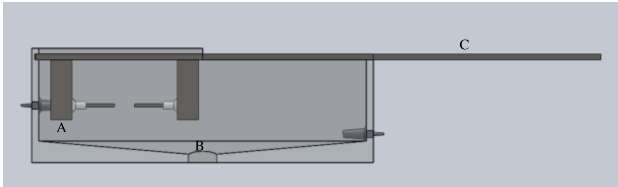
Figure 14: Lunchbox Design with sliding Luer connection (A), sloped bottom for draining media (B), and sliding lid with long handle (C).
