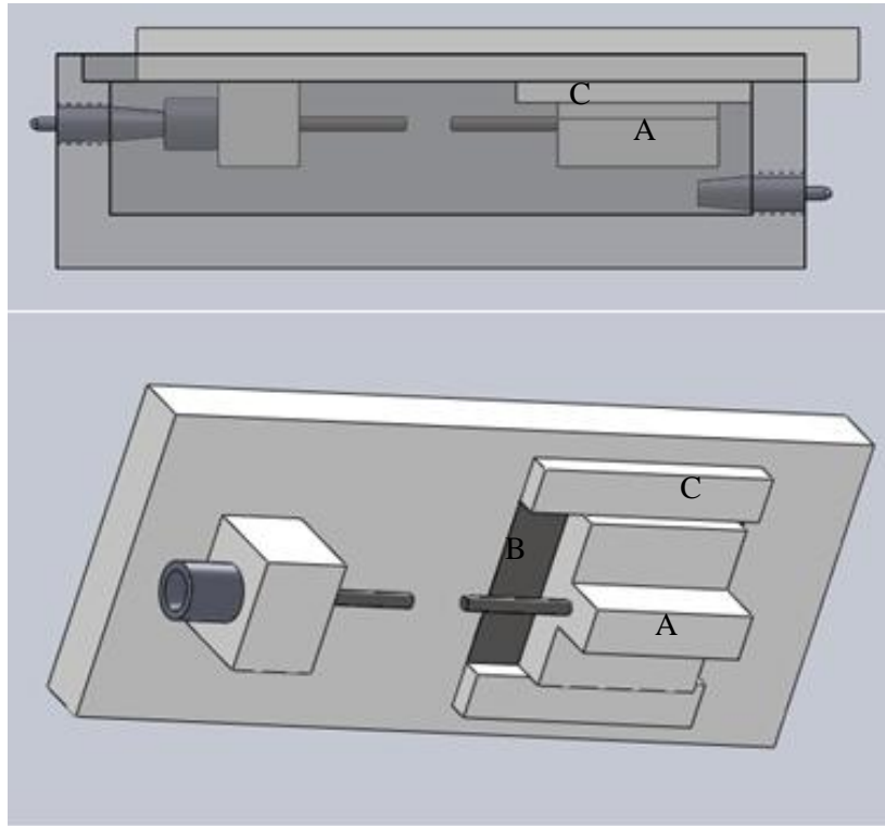
Figure 17: The magnetic track design includes a moveable arm with an embedded magnet (A). The lid had an embedded steel plate (B) with ridges along the side for guidance (C).
