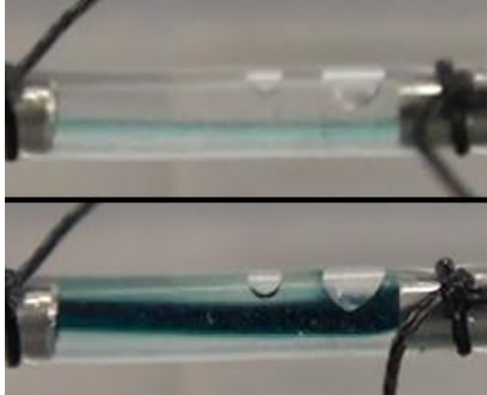
Figure 38: Laminar flow shown by upstream injection of food coloring. This image shows a thin stream (A) as well as a thick stream (B) showing no signs of turbulent flow.
