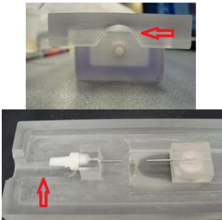
Figure 59: Top picture: Arc cutout on the lid around the inlet Luer connector. Bottom Picture: Arc depression in the lid.
