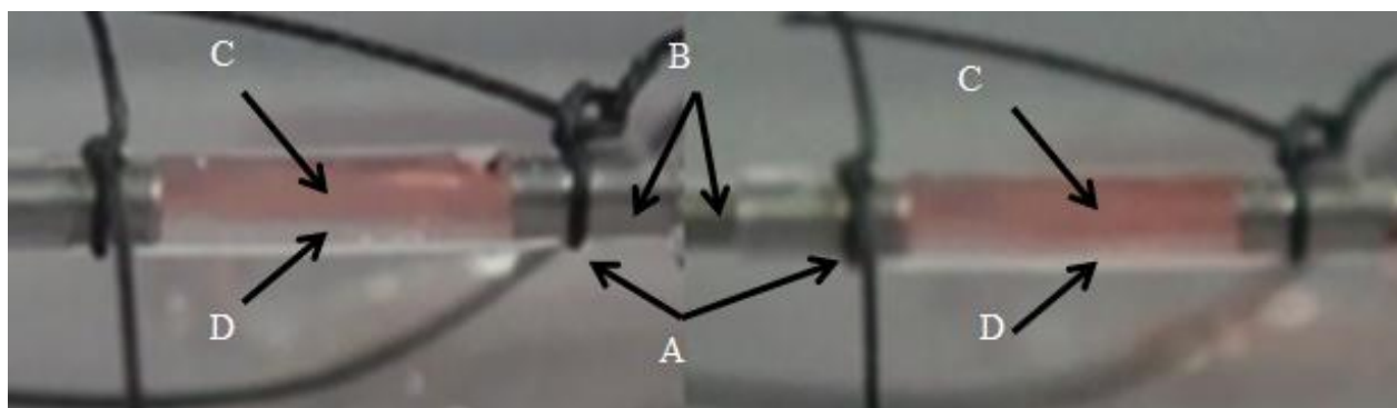
Figure 36: The silicone tubing is sutured (A) to the syringe needles (B). The red food coloring makes a visible, distinct layer (C) above the clear water (D).
