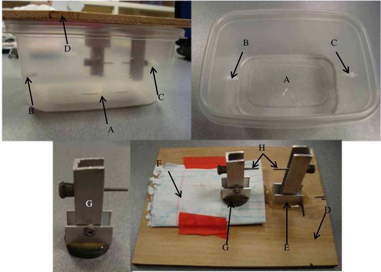
Figure 18: The initial prototype consisted of a Tupperware® container (A) with outlet (B) and inlet (C) Luers, a wooden board (D) acting as the lid with a stationary aluminum arm (E) and steel track (hidden by the paper labeled by F), and a magnetic aluminum movable arm (G). Both arms have aligned syringe needles (H). The paper was used to even out the height of the movable arm.
