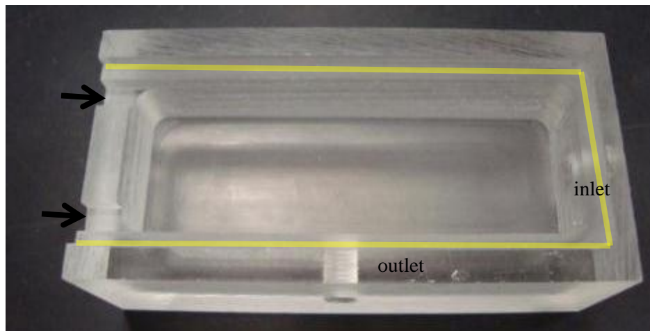
Figure 21: Acrylic prototype chamber with edges for lid (highlighted in yellow) and slots for ridges on lid (labeled with arrows).
