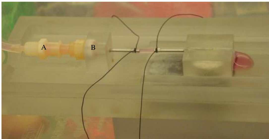
Figure 33: Female Luer connector (A) attached to the stationary arm (B) to complete flow loop when lid is being tested.
