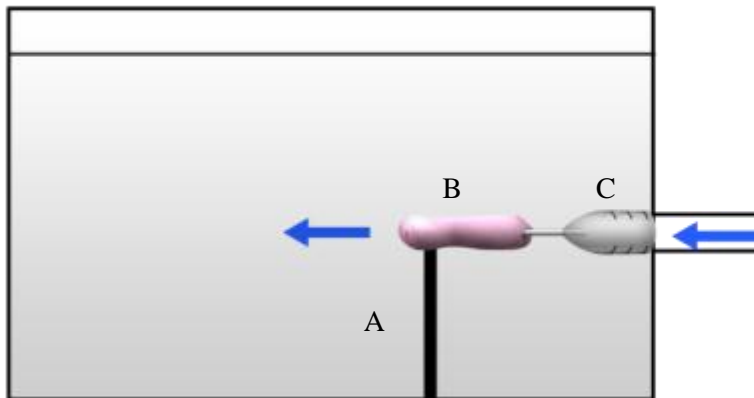
Figure 11: Open Cartridge Design 2 consists of plastic supports connected to a syringe needle (A) to hold the end of the tissue tube (B) while a syringe needle on the inlet (C) holds the other end.
