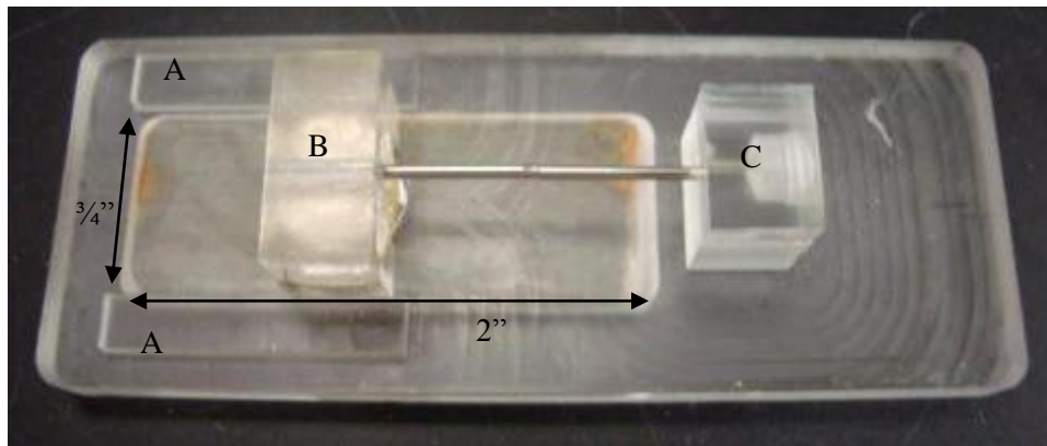
Figure 22: Acrylic prototype lid consisting of ridges (A) for the moveable arm (B) and a stationary arm (C). Arrows indicate the dimensions of the depression for the steel piece.
