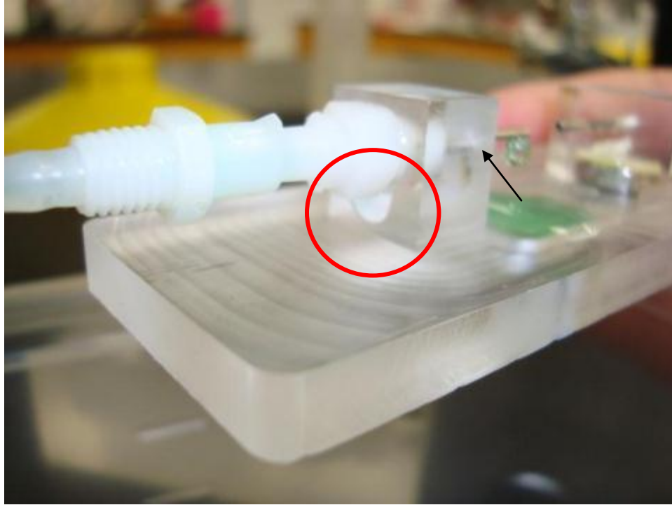
Figure 24: Leak around threading of the stationary arm (circle). No leaking was observed at the stationary arm-syringe needle interface (arrow).
