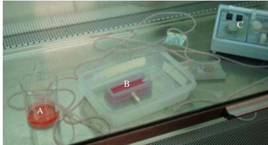
Figure 31: (A) Beaker containing media, (B) bioreactor chamber in plastic tray, and (C) pump being set up under a sterile fume hood.
