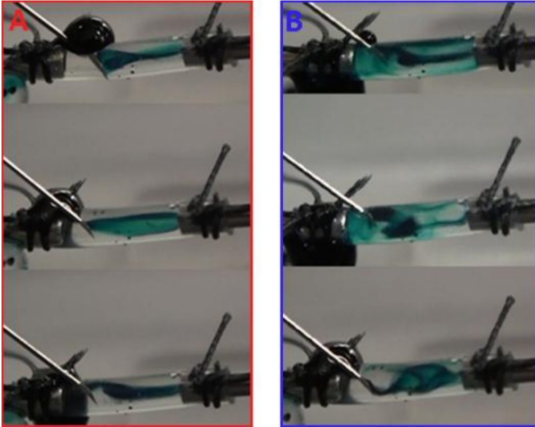
Figure 37: Flow patterns that resembled laminar flow (A) and turbulent flow (B).
