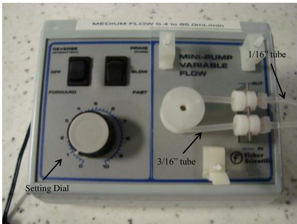
Figure 23: Fisher Scientific peristaltic pump with flow rates ranging between 0.4-85.0mL/min.
