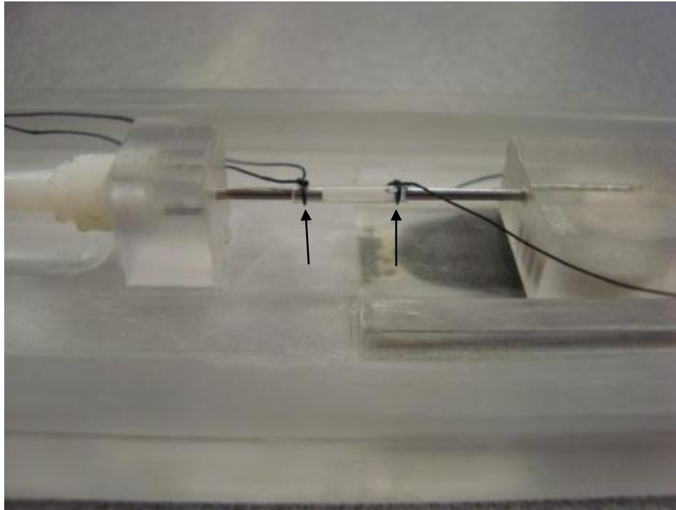
Figure 30: Silicone tube mounted onto the syringe tips using medical sutures (arrows).
