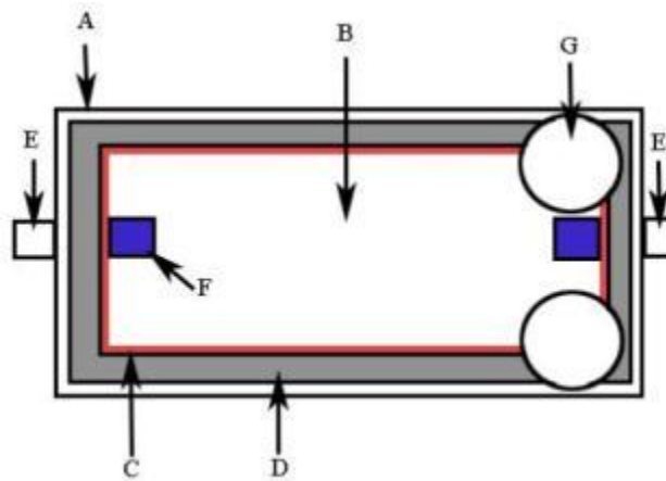
Figure 4: Growth cassette developed by Webb et al. (2007) which includes the cassette body (A), plexiglass faceplate (B), rubber gasket (C), aluminum frame (D), flow inlet/outlets via Luer connectors (E), Luer connector for scaffold attachment (F), and an air filter for gas exchange attached to a Luer connector (G).
