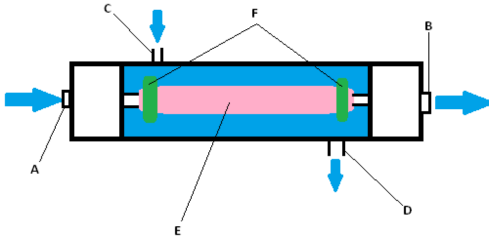
Figure 5: Bioreactor made by Zhang et al. (2009). Labeled are (A) luminal inlet, (B) luminal outlet, (C) external media inlet, (D) external media outlet, (E) silk-based vascular graft, and (F) the O-rings which hold the graft in place.
