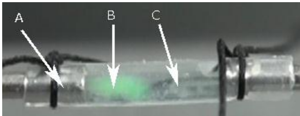
Figure 26: Silicone tubing (ID 1.47mm) was sutured to the syringe needles (A). Both large (B) and small (C) particles are seen flowing through the tubing.
