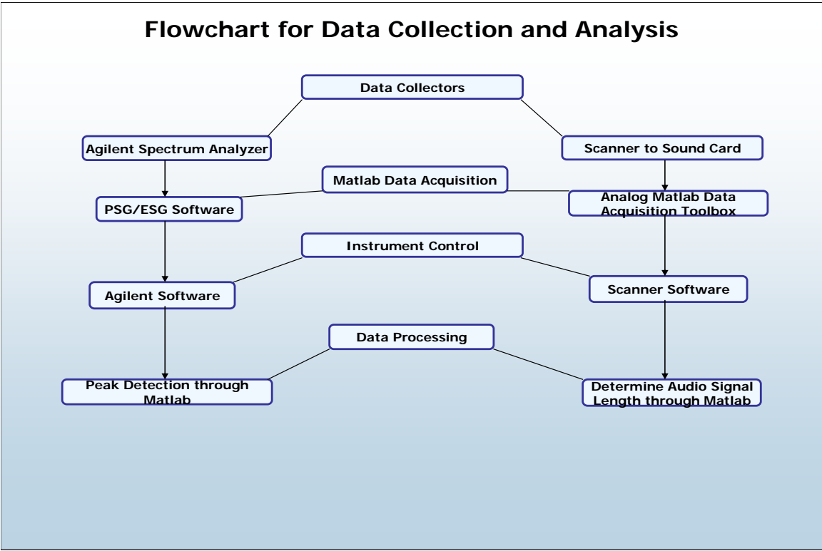
Figure 7 - Project Flowchart
