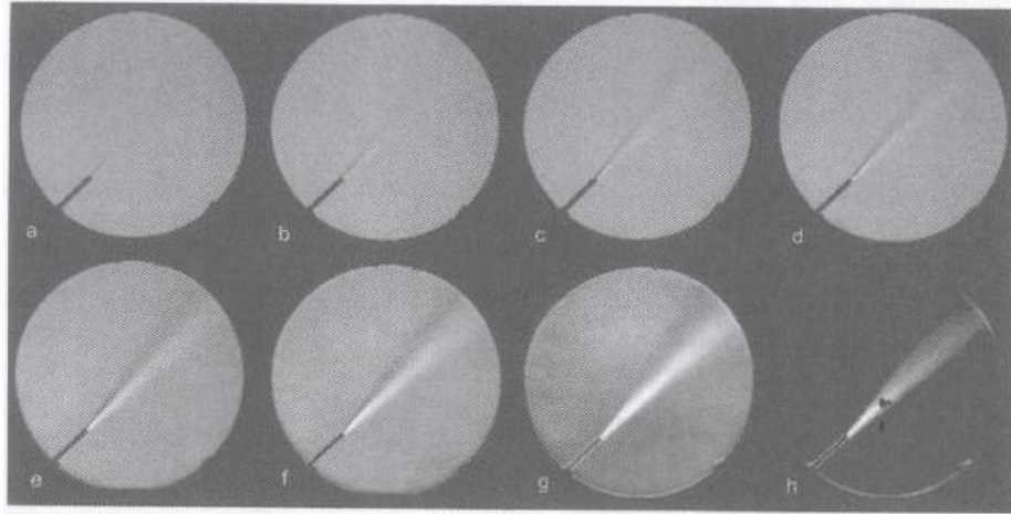
Figure 36: Schlieren image of a gas jet at a) 0%, b) 20%, c) 40%, d) 60%, e) 80%, f) 90%, g) 95%, and h) 100% of the measuring range (Ref [17] © 2001, Springer)
