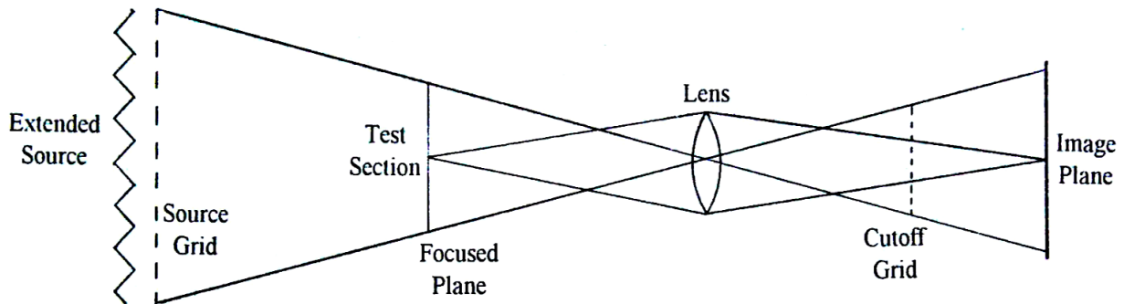
Figure 33: A focusing schlieren system arrangement (Ref [20] © 2006, Hanenkamp)
