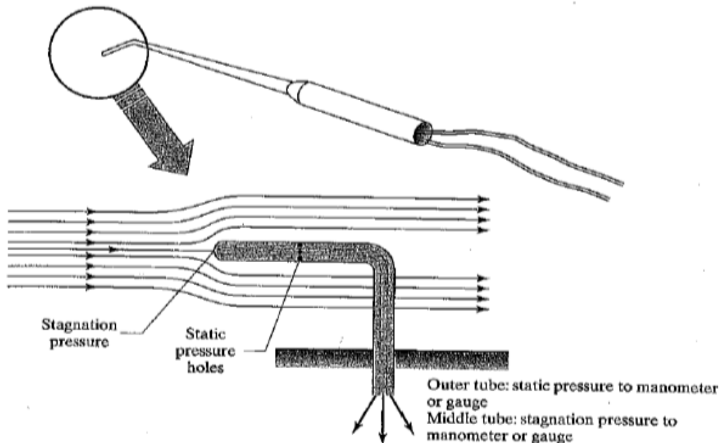
Figure 15: Pitot-static tube [14]
