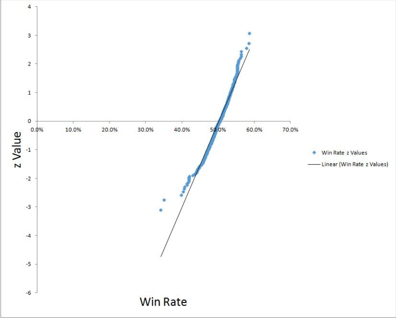
Figure 26: Normal Probability Plot for Support Win Rate
