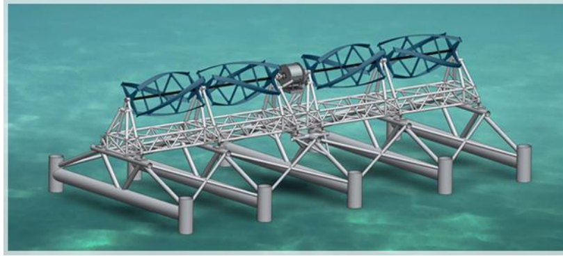
Figure 40: TiGen Power System
