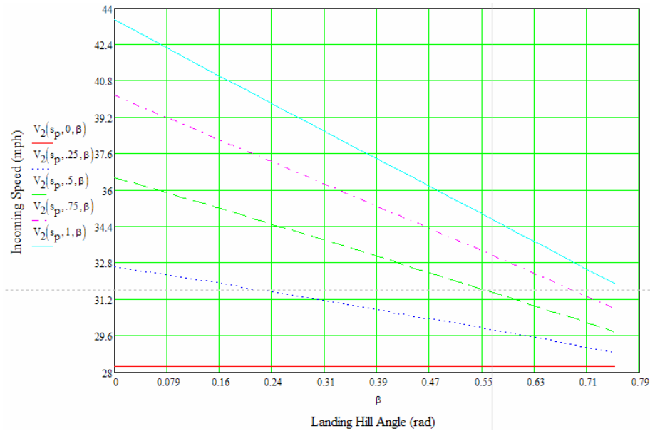
Figure 5-4: Landing Hill Angles v. Necessary Speed, Varying % Landing Downhill
