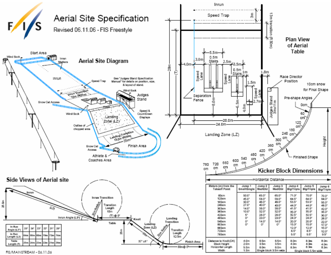
Figure 2-3: Aerial Site Specifications
