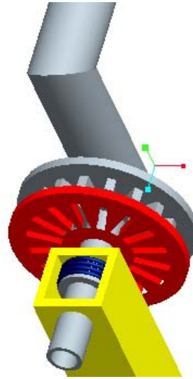
Figure 7: Unlocked Position
