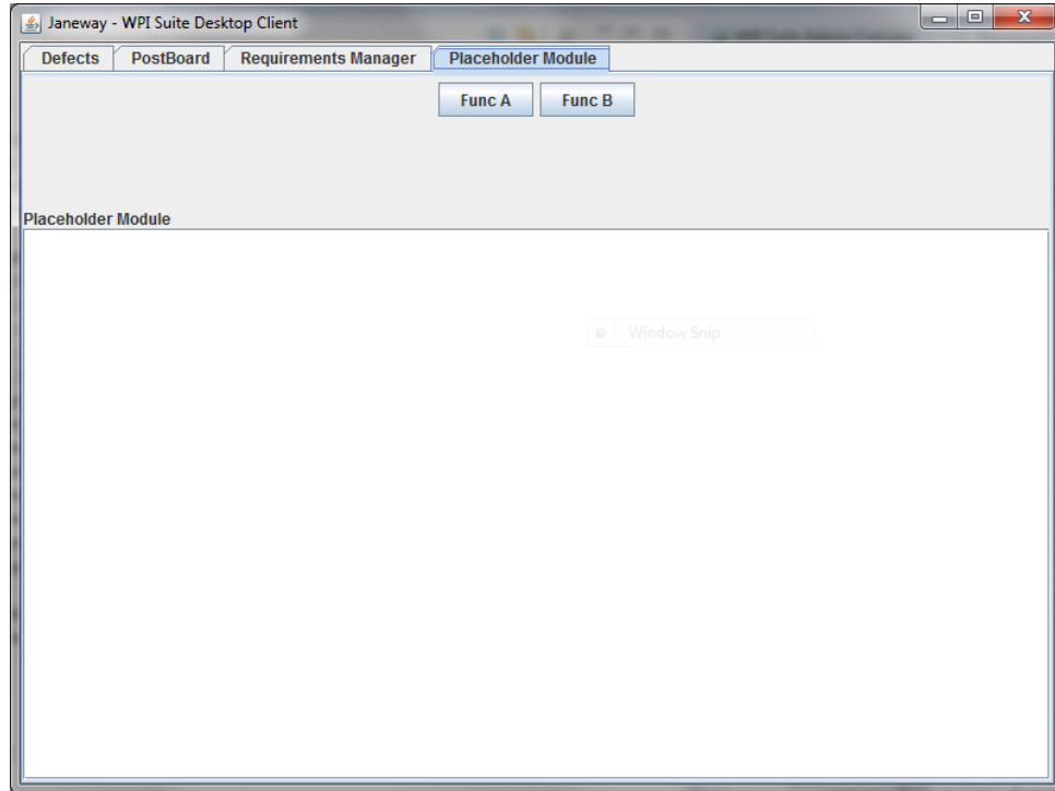
Figure 11: Janeway GUI
