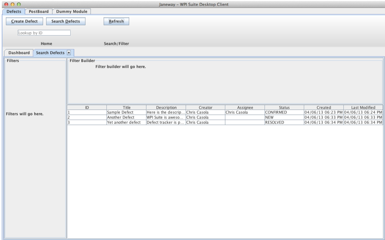
Figure 17: Browse Defects
