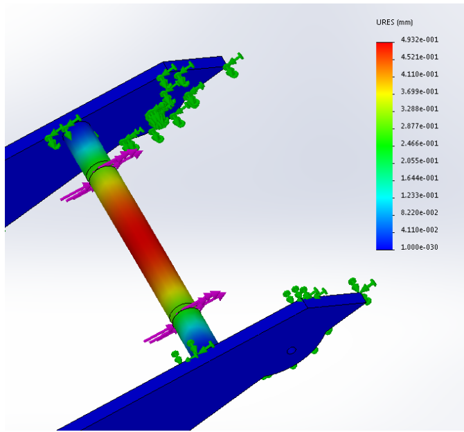
Figure 29: The expected deflection of a piece of rigid PVC tubing.
