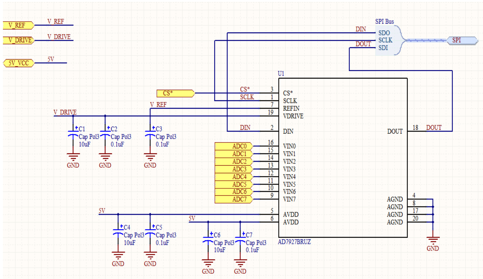
Figure 4.2.13: Schematic Setup for the Selected Analog to Digital Converter
