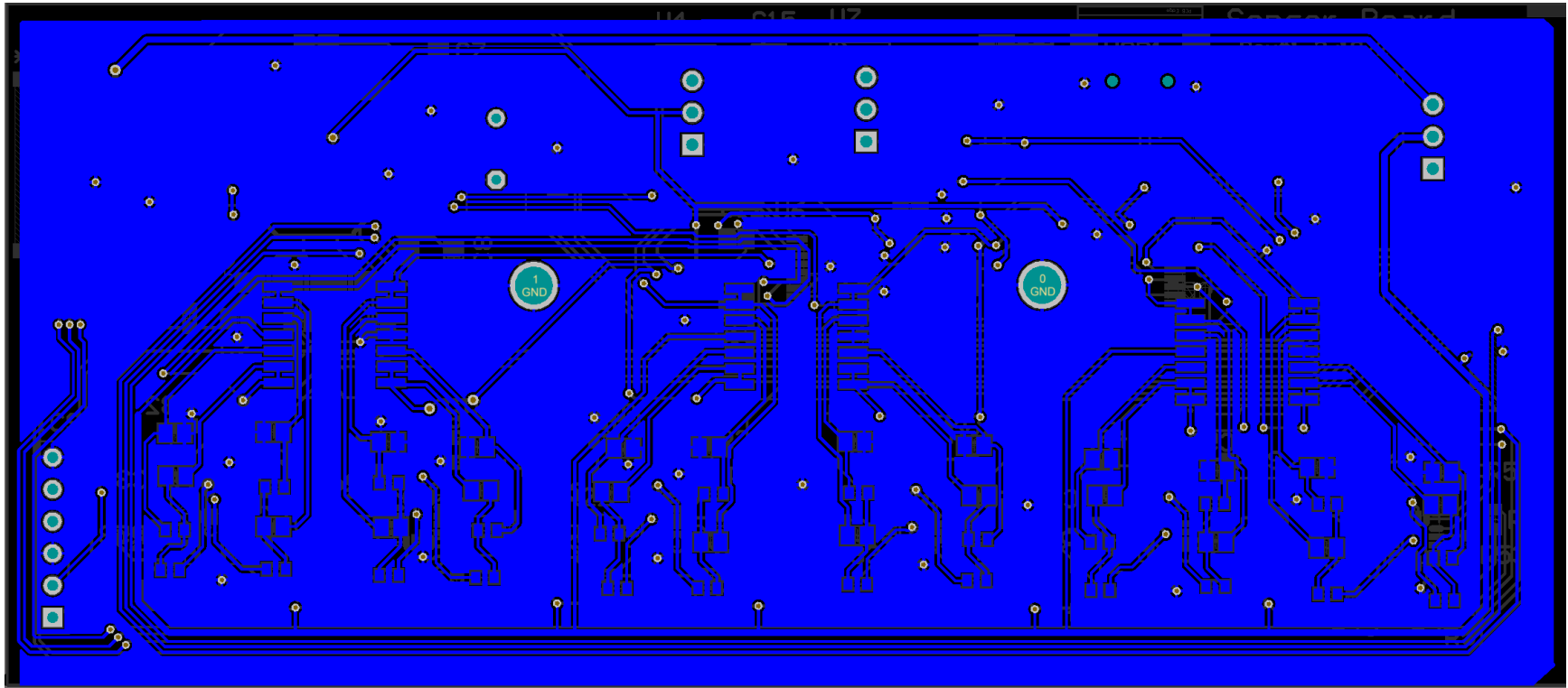
Figure D.2: Sensor Board PCB, Altium Rear View
