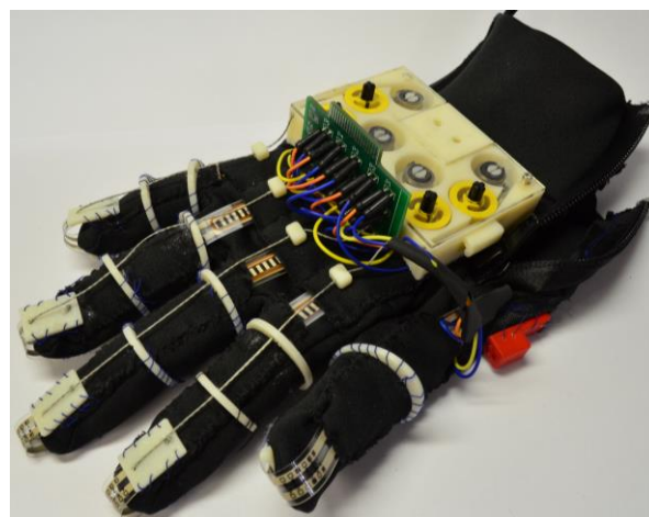
Figure A: Fully Assembled Exomuscular Glove with Flex and Pressure Sensors.
