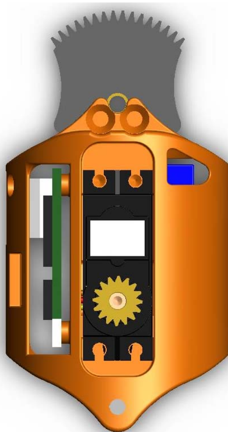
Figure 32: Final Design Bottom
