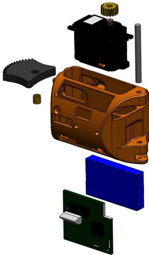
Figure 33: Vertebrae Assembly Exploded View
