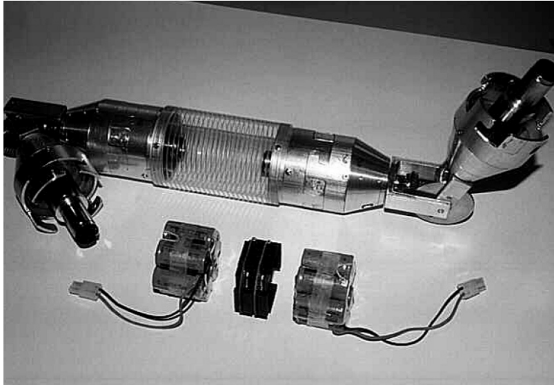
Figure 8: Nilsson's Universal Serpentine Link
