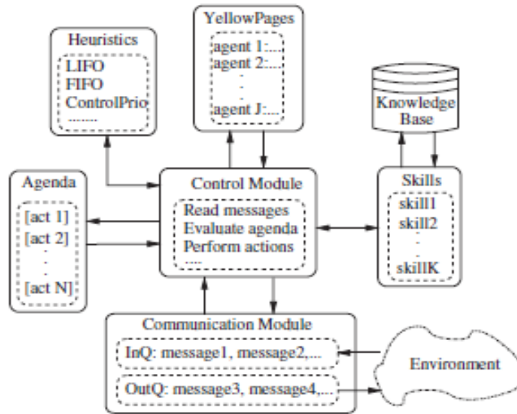
Figure 8: Skeleton Agent Architecture
