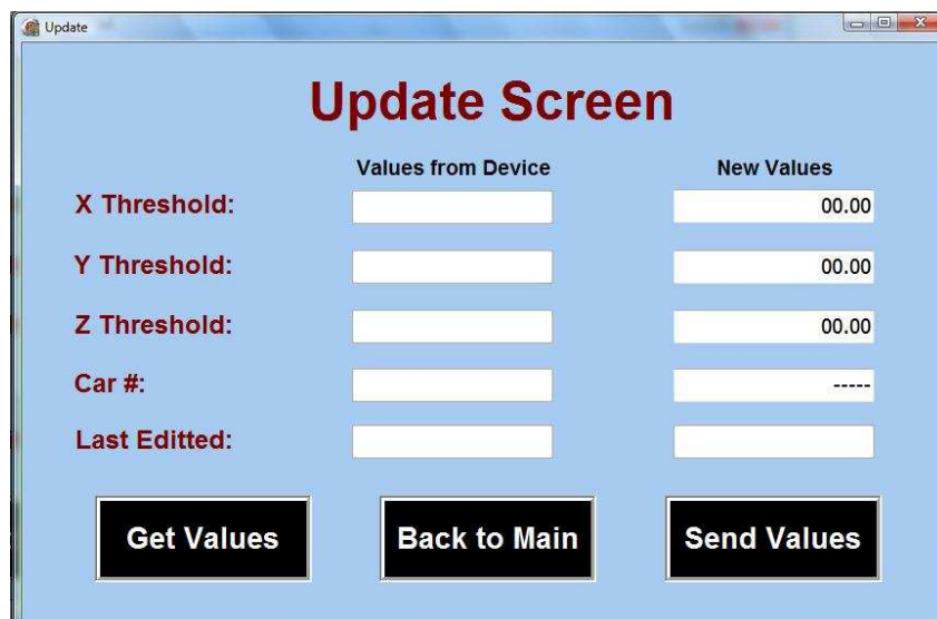
Figure 32: Update Screen
