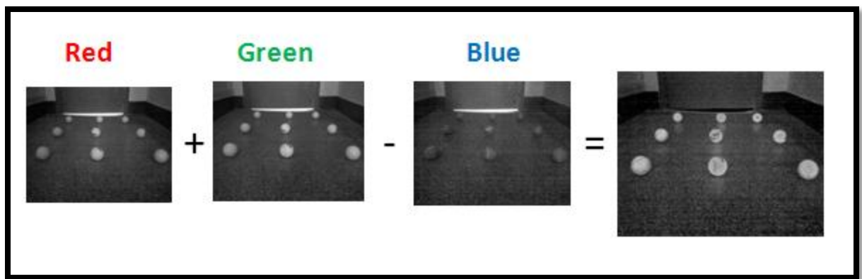
Figure 27: Optimal Colorization
