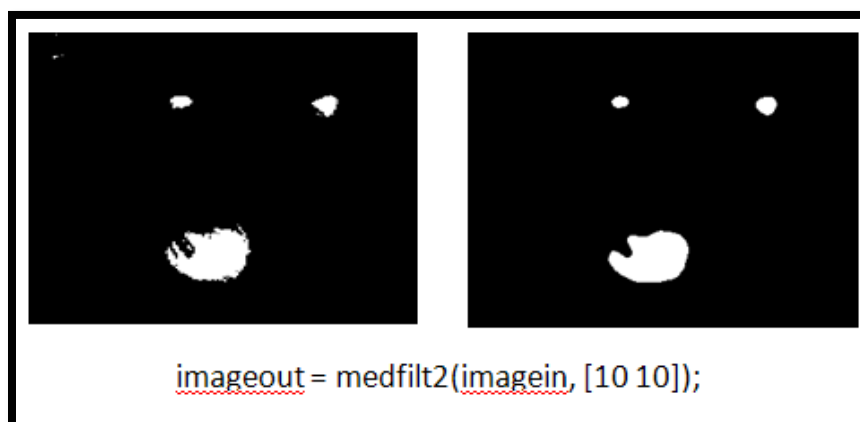
Figure 36: Median Filtration
