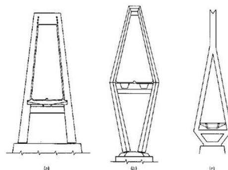
Figure 40: Tower Configurations
