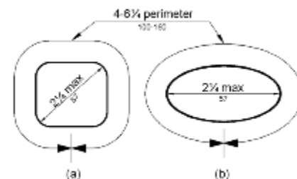
Figure 20: Noncircular Handrail Cross Sections
