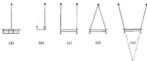
Figure 39: Transverse Cable Arrangements
