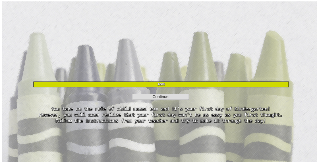
Figure 4.3: Loading Screen
