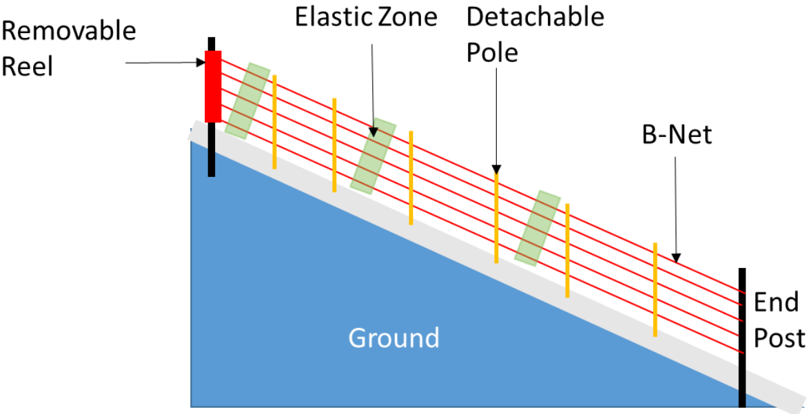
Figure 4: Diagram of the design result
