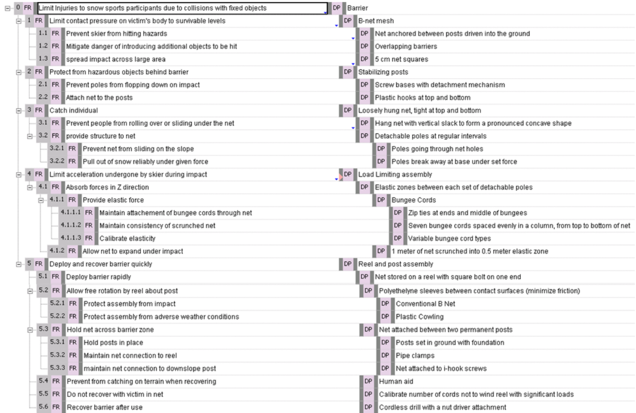
Figure 24: Full Energy Absorbing Barrier Decomposition
