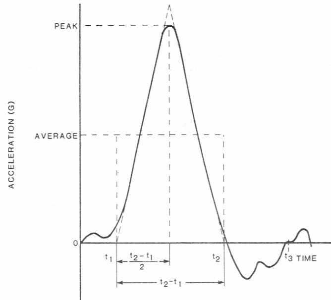
Figure 17: Acceleration vs Time (Shanahan, 2004)
