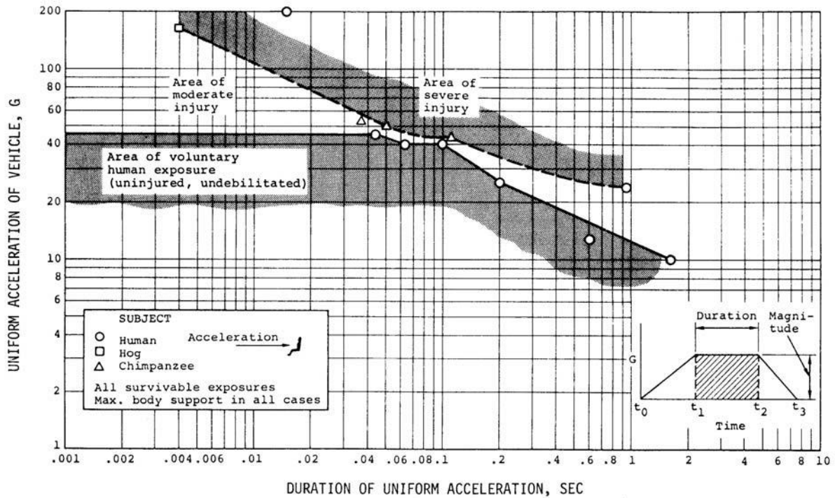
Figure 18: Acceleration Injury Criteria (Shanahan, 2004)
