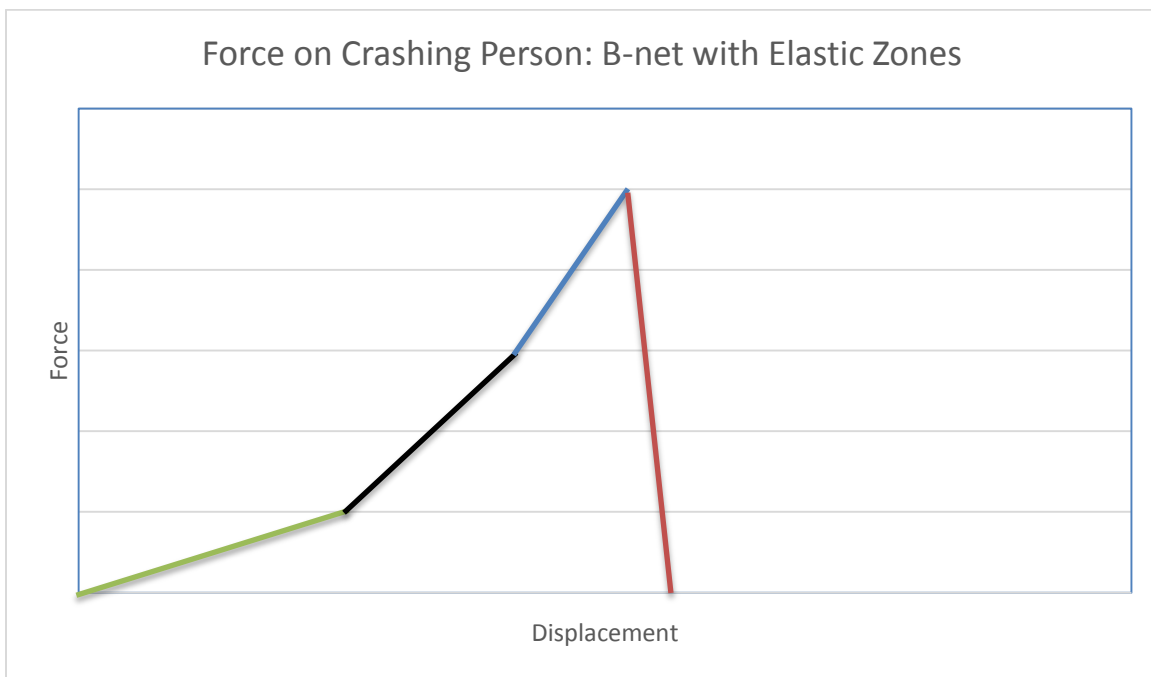
Figure 10: Crash Forces on Modified B-net
