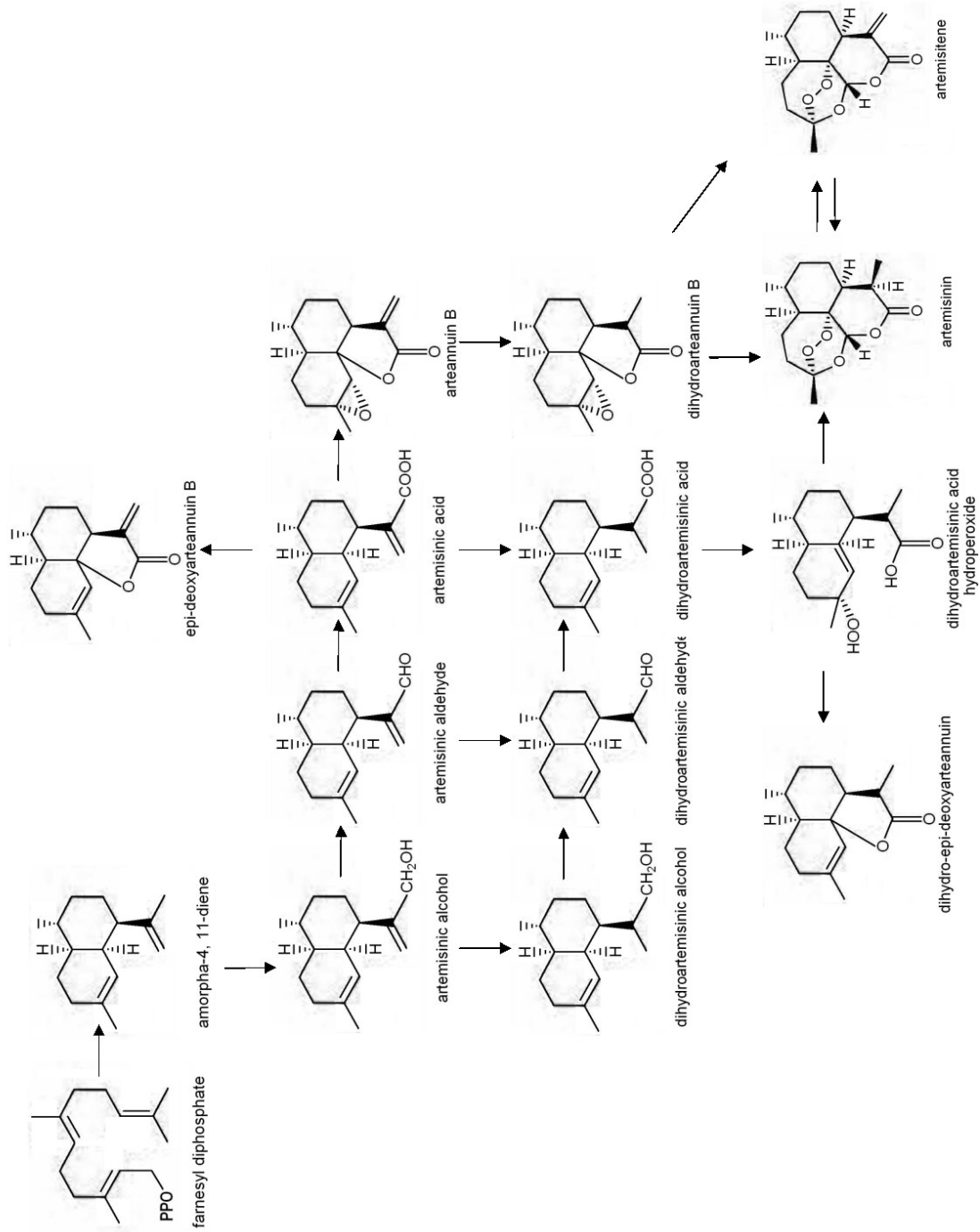
Figure 2: Proposed biosynthetic pathway of artemisinin – A composite of the pathways proposed by Wallart et al. 2000, Abdin et al. 2002 and Bertea et al. 2005.
