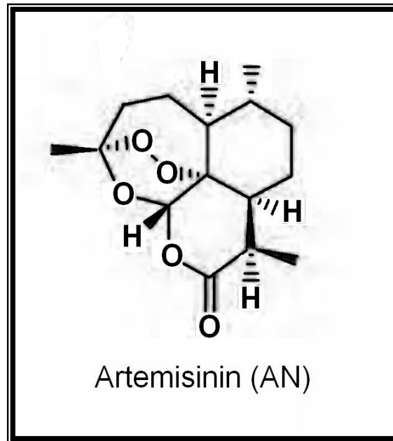
Figure 1: The chemical structure of Artemisinin
