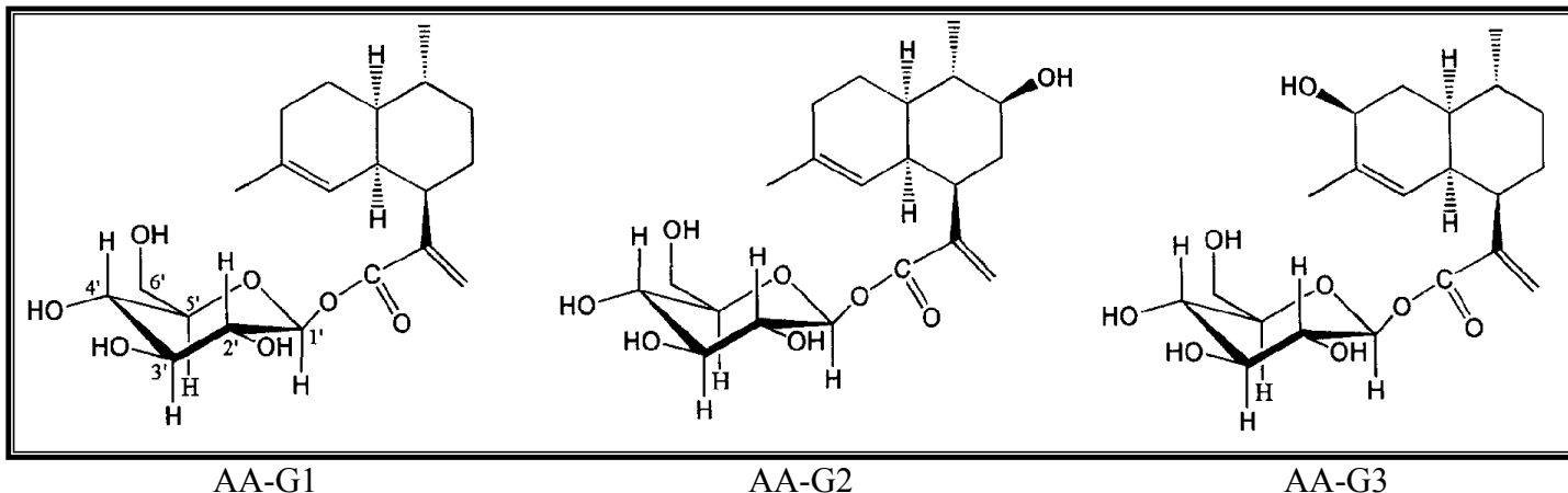
Figure 3: The biotransformation products of artemisinic acid:
