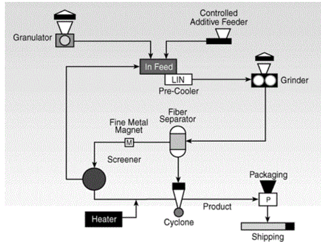
Figure 10 - Cryogenic Grinding Process (Tire Recycling Made Simple, 2012).
