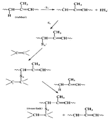
Figure A21 - The Vulcanization Process (Li & Fox, 2012)
