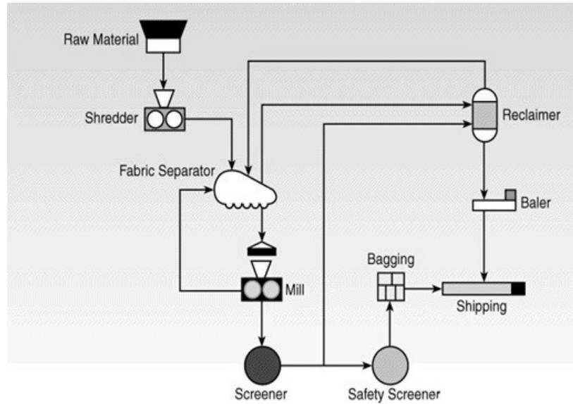
NOTE: Magnets are used throughout the process Figure 9 - Ambient Grinding Process (Tire Recycling Made Simple, 2012).
