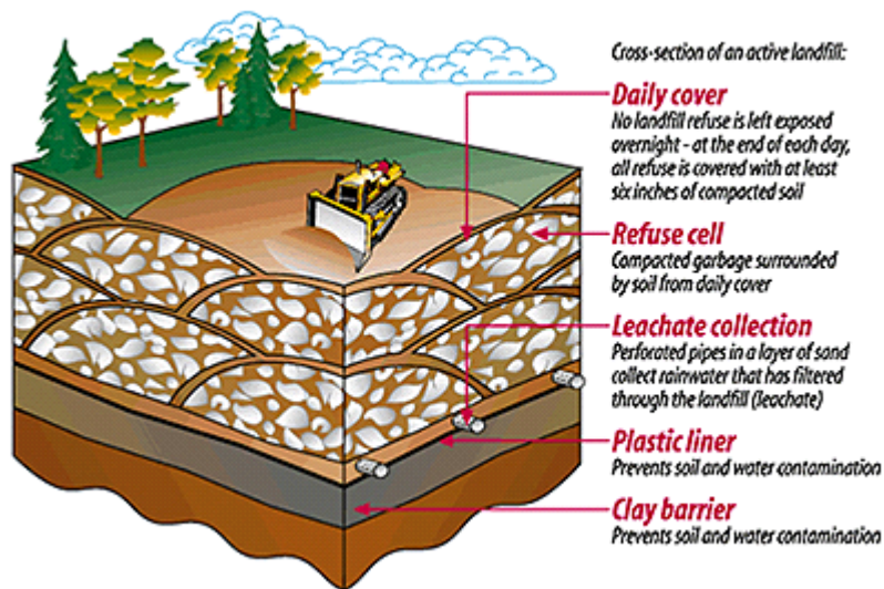
Figure 6 - Schematic representation of a sanitary landfill (South Kent Landfill, 2012).
