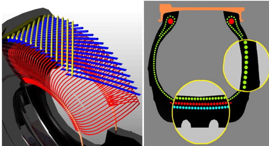
Figure D1 - Radial Tire ( Radial versus Bias Technology , 2012).
