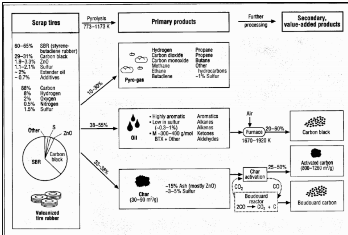
Figure 7 - The products obtained from pyrolysis (Wojtowicz & Serio, 1996).
