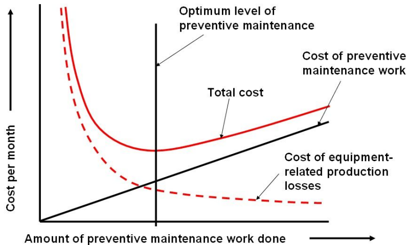
Figure 8: Maintenance Cost Curve (Veleda, 2018)
