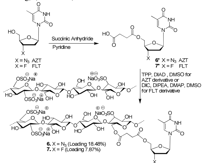
Scheme 2. Synthesis of AZT-succinate-CS ( 6 ) and FLT-succinate-CS ( 7 ) conjugates.
